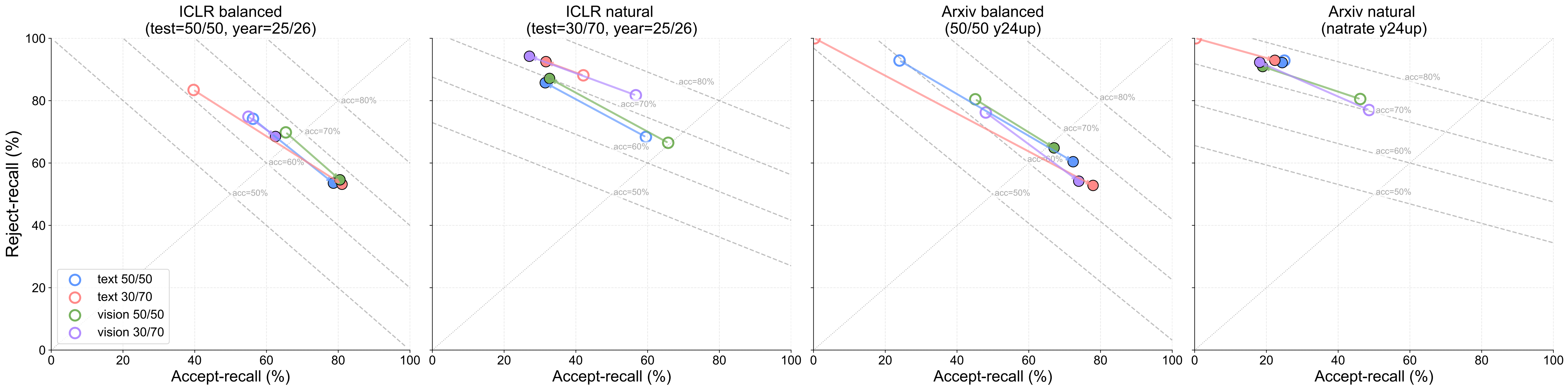
Per-class recall: raw (open) → calibrated (filled) — 7B, TEST split
