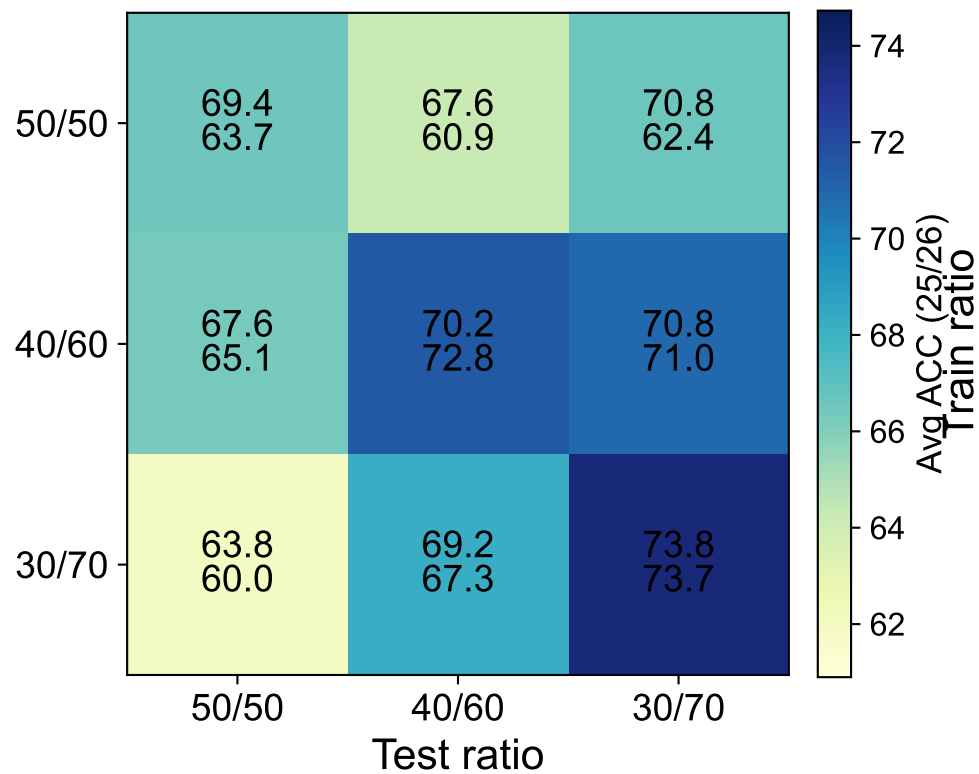
Raw ACC (no calibration)
