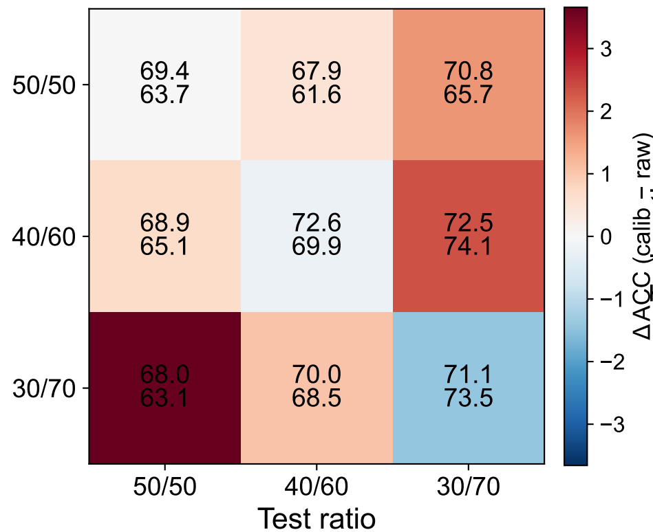
Calibrated ACC ( \Delta from raw)
