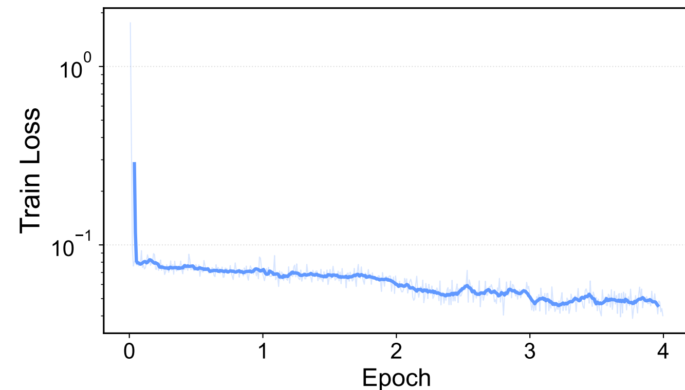
Train Loss — 40/60
