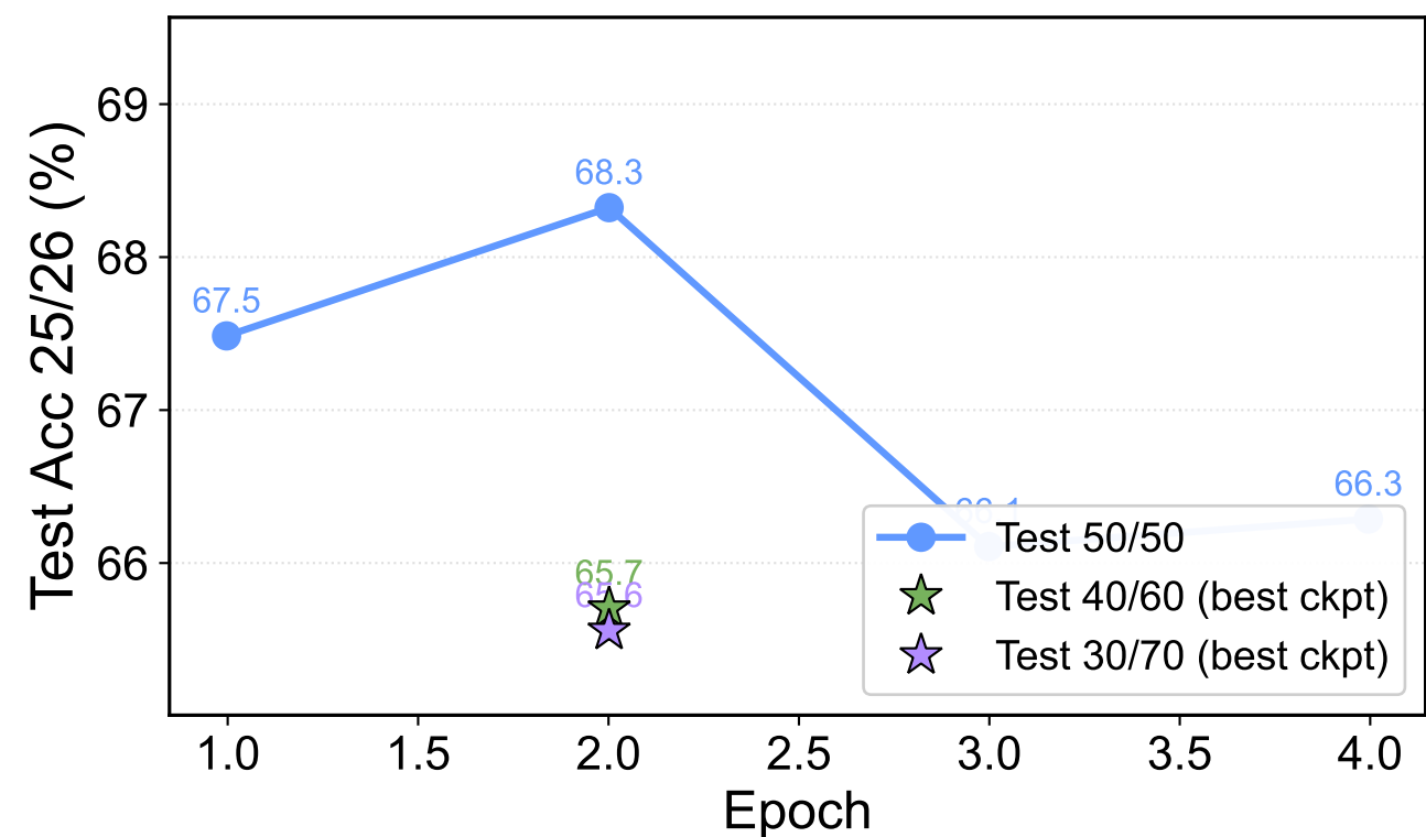
Test Acc 25/26 — 40/60
