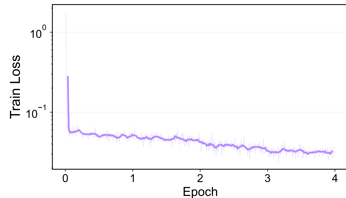
Train Loss — 30/70
