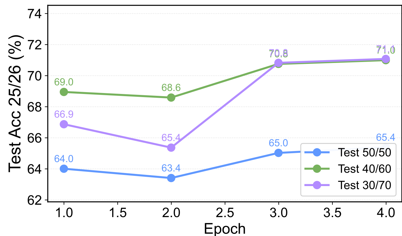
Test Acc 25/26 — 30/70
