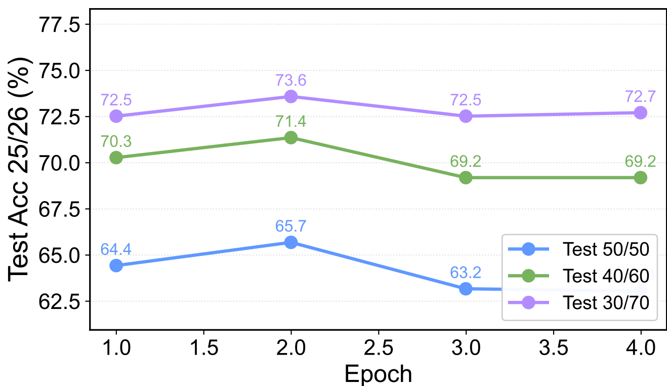
Test Acc 25/26 — 30/70
