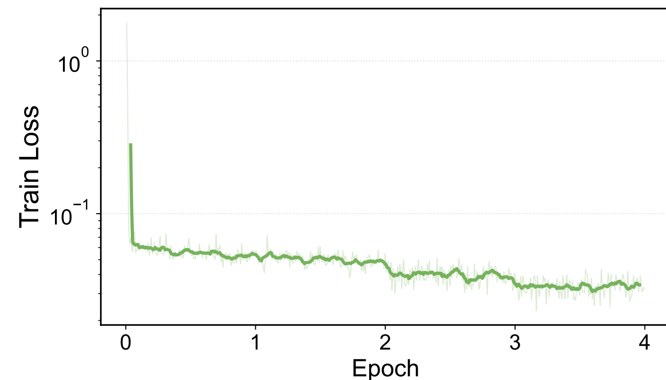
Train Loss — 30/70
