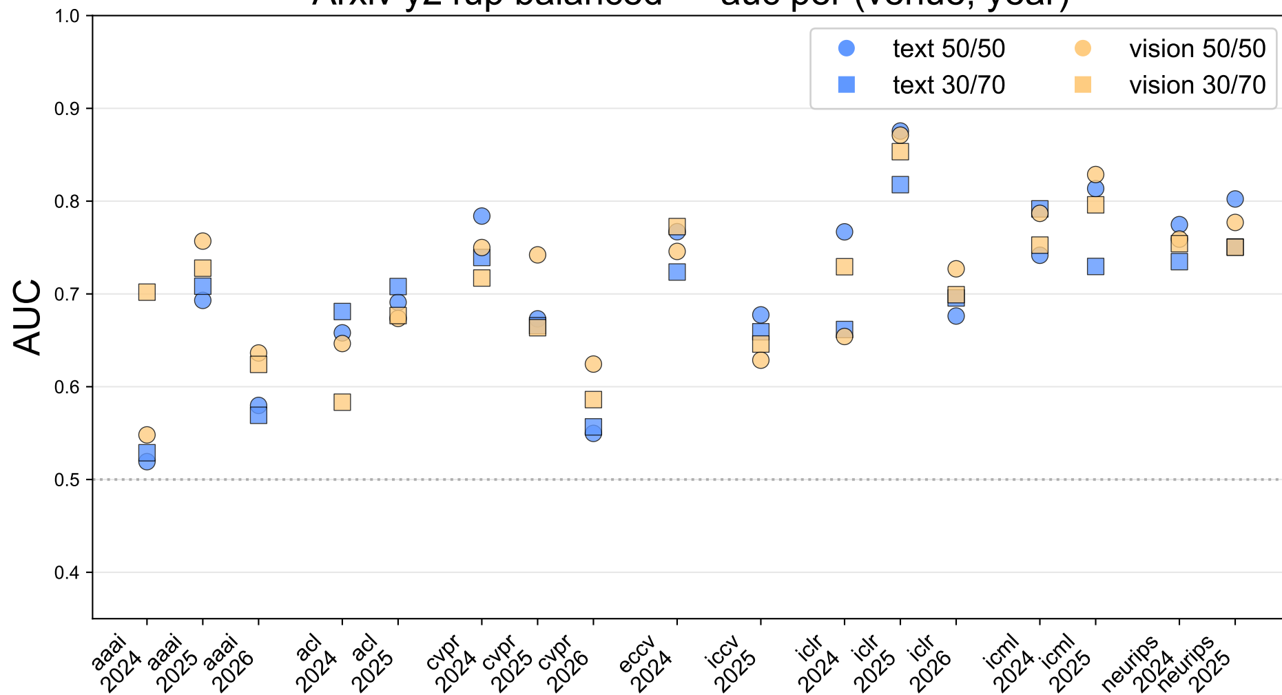
Arxiv y24up balanced — auc per (venue, year)
