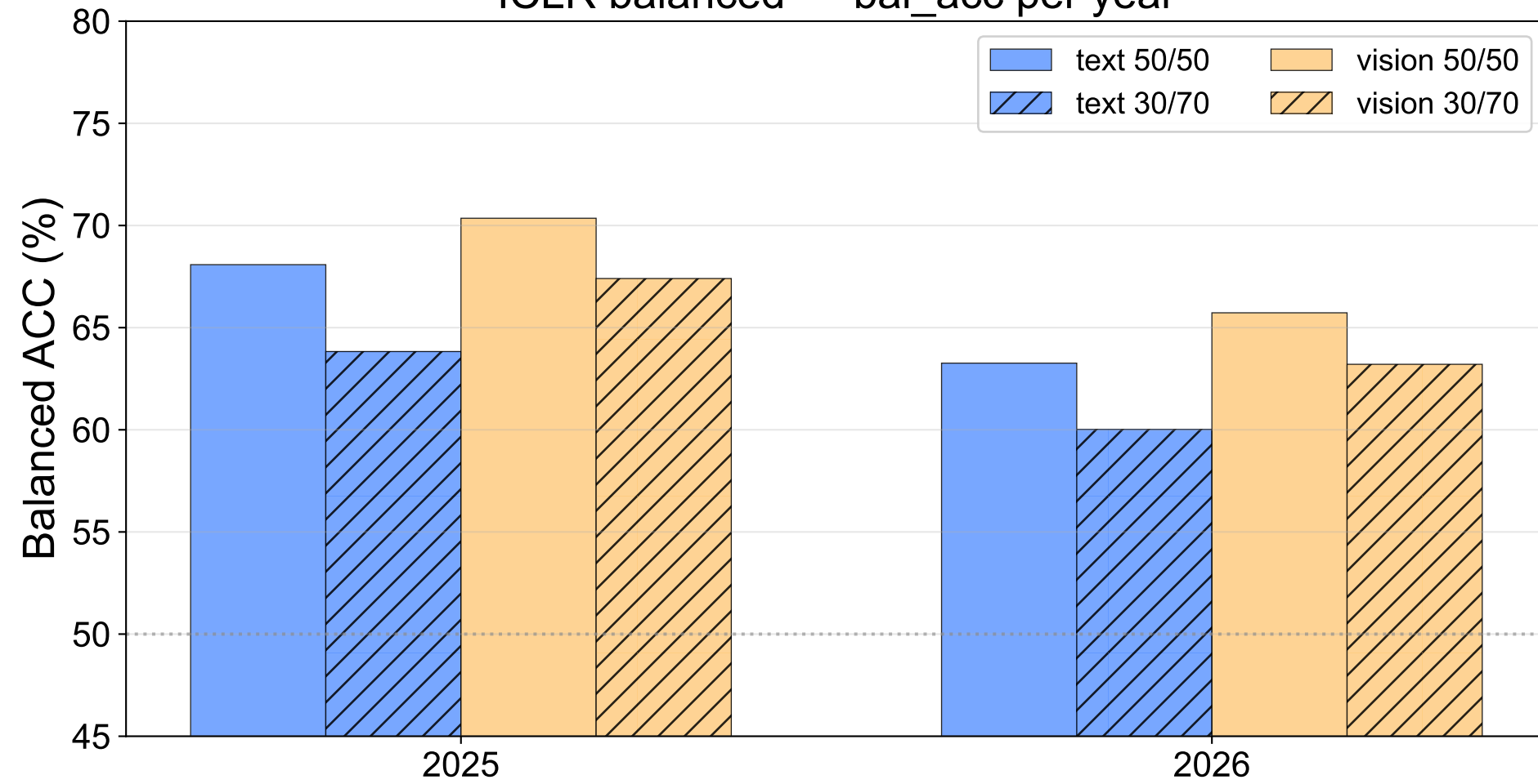
ICLR balanced — bal_acc per year
