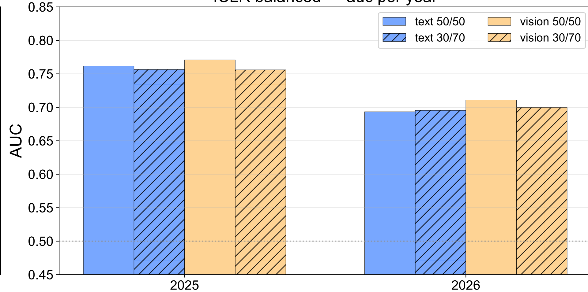
ICLR balanced — auc per year
