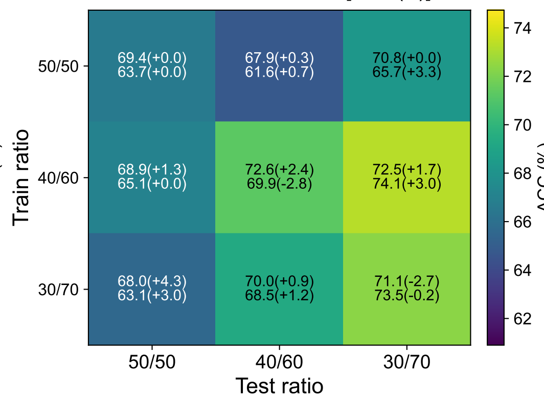
ICLR Calibrated ACC [calib( \Delta )]
