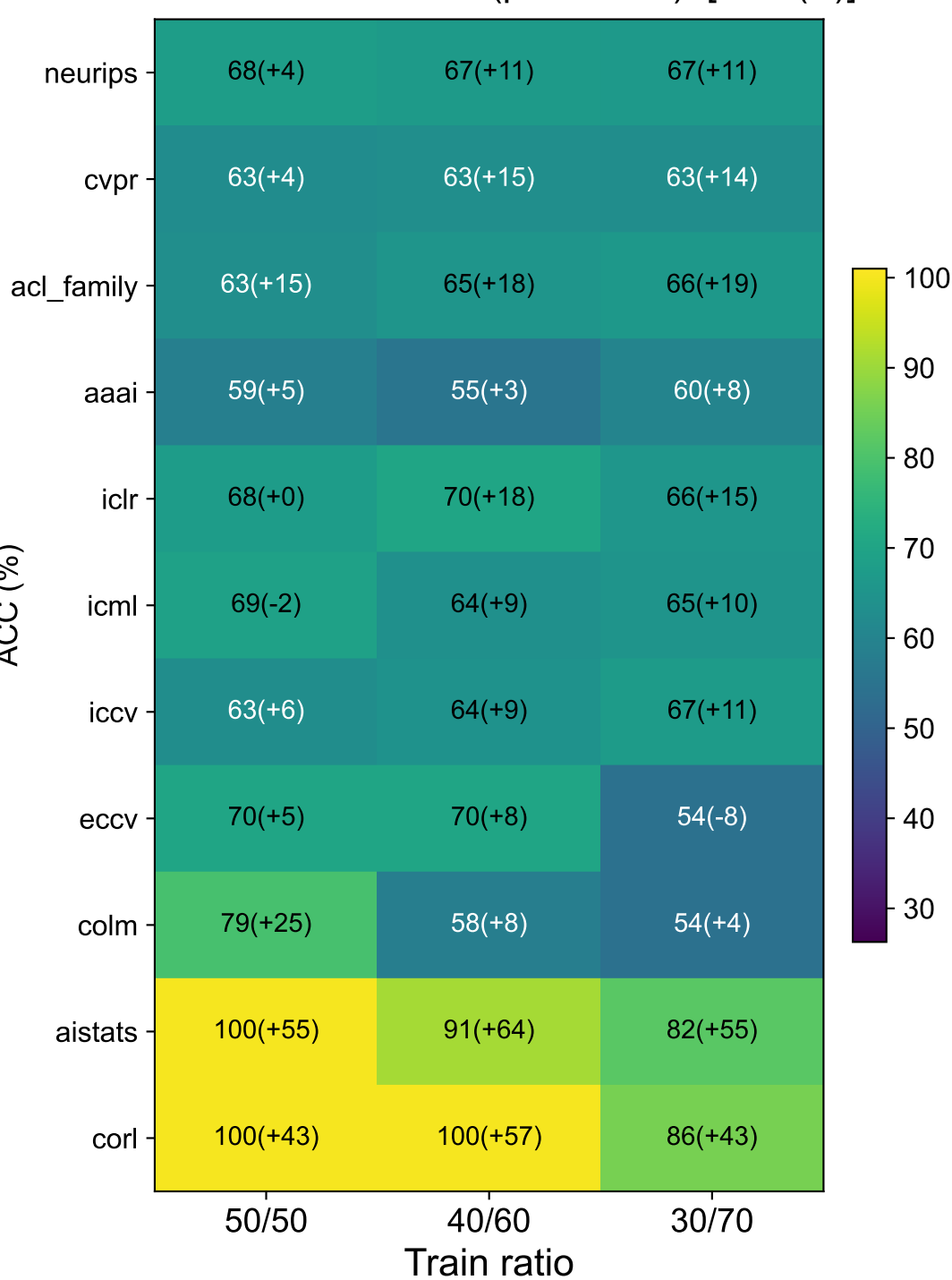
Arxiv Calibrated ACC (per venue) [calib( \Delta )]
