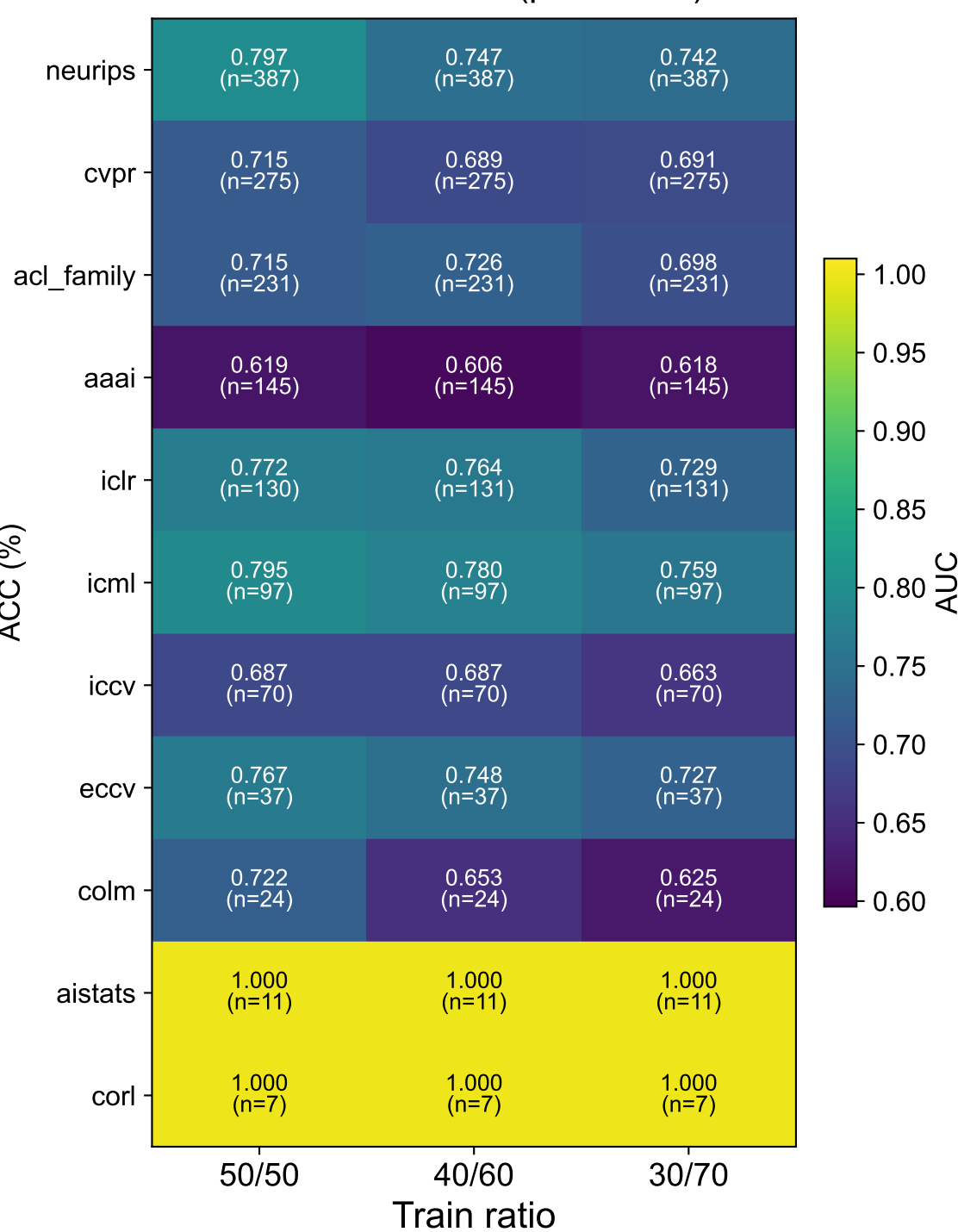
Arxiv ROC-AUC (per venue)
