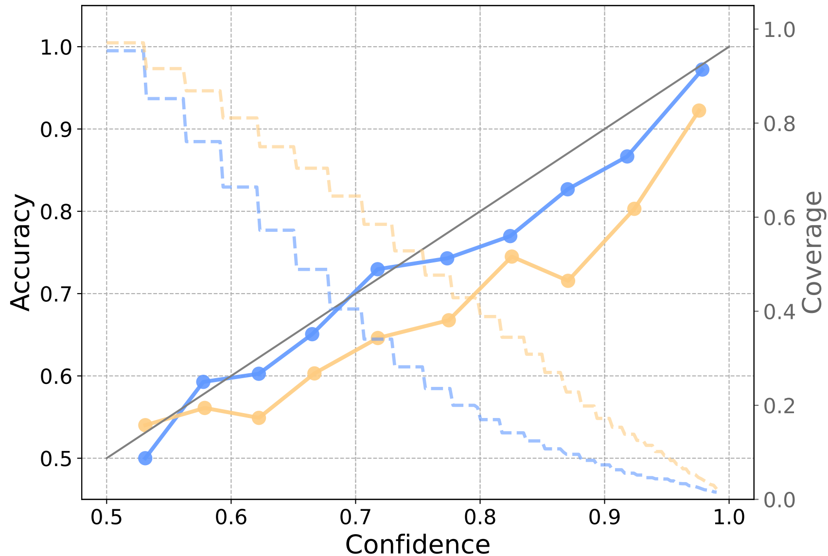
(a) Per-Bin Reliability (10 bins, width=0.05)
