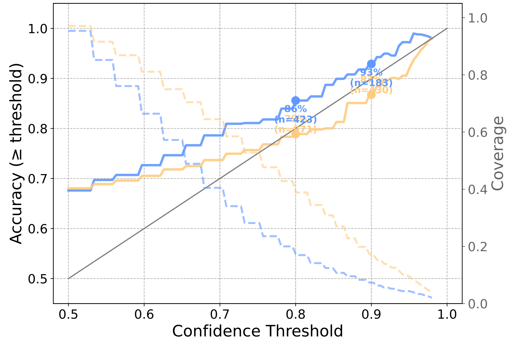
(b) Cumulative Accuracy ( \geq threshold)
