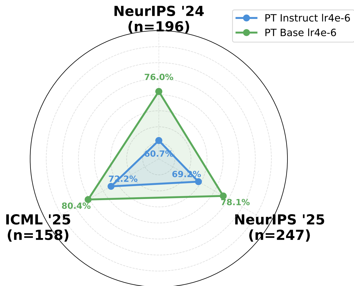
(b) Midtrain + SFT — Accept Recall
