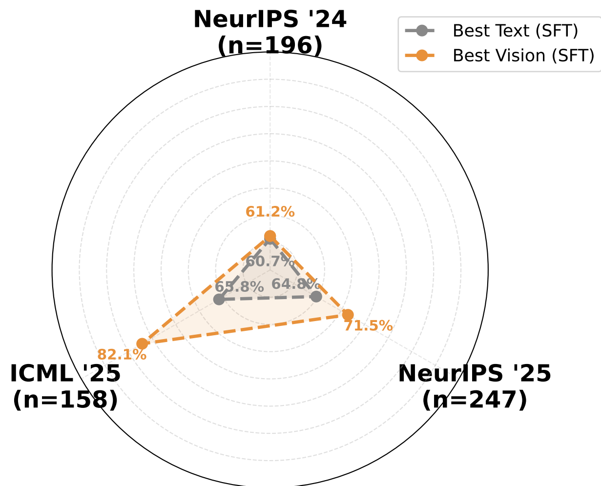
(a) SFT-only — Accept Recall
