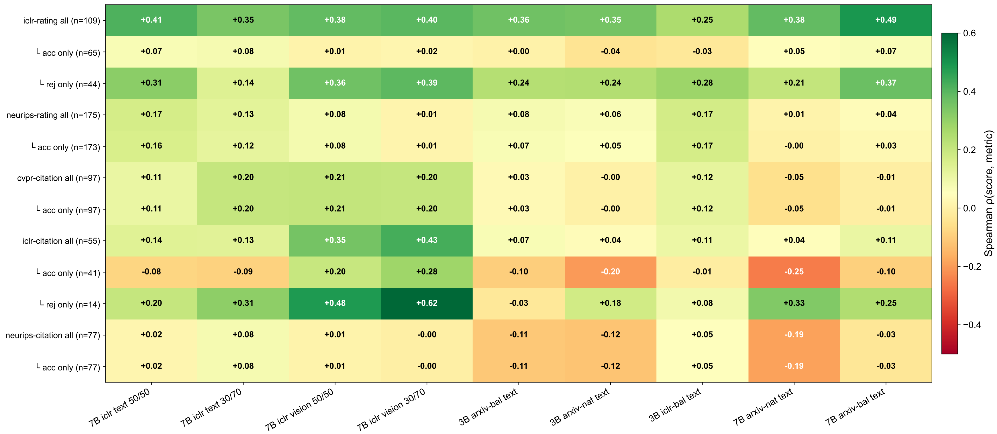
Per-(venue, metric) Spearman \rho — within-class decomposition \rho_{\text{all}} = combined; \rho_{\text{acc}}/\rho_{\text{rej}} = within-class (separates binary signal from quality discrimination)
