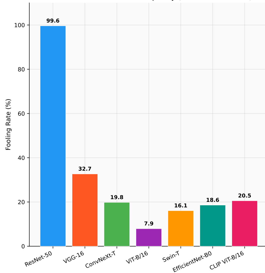
Transfer Fooling Rate CNN→Transformer transfers poorly (ViT most resistant)
