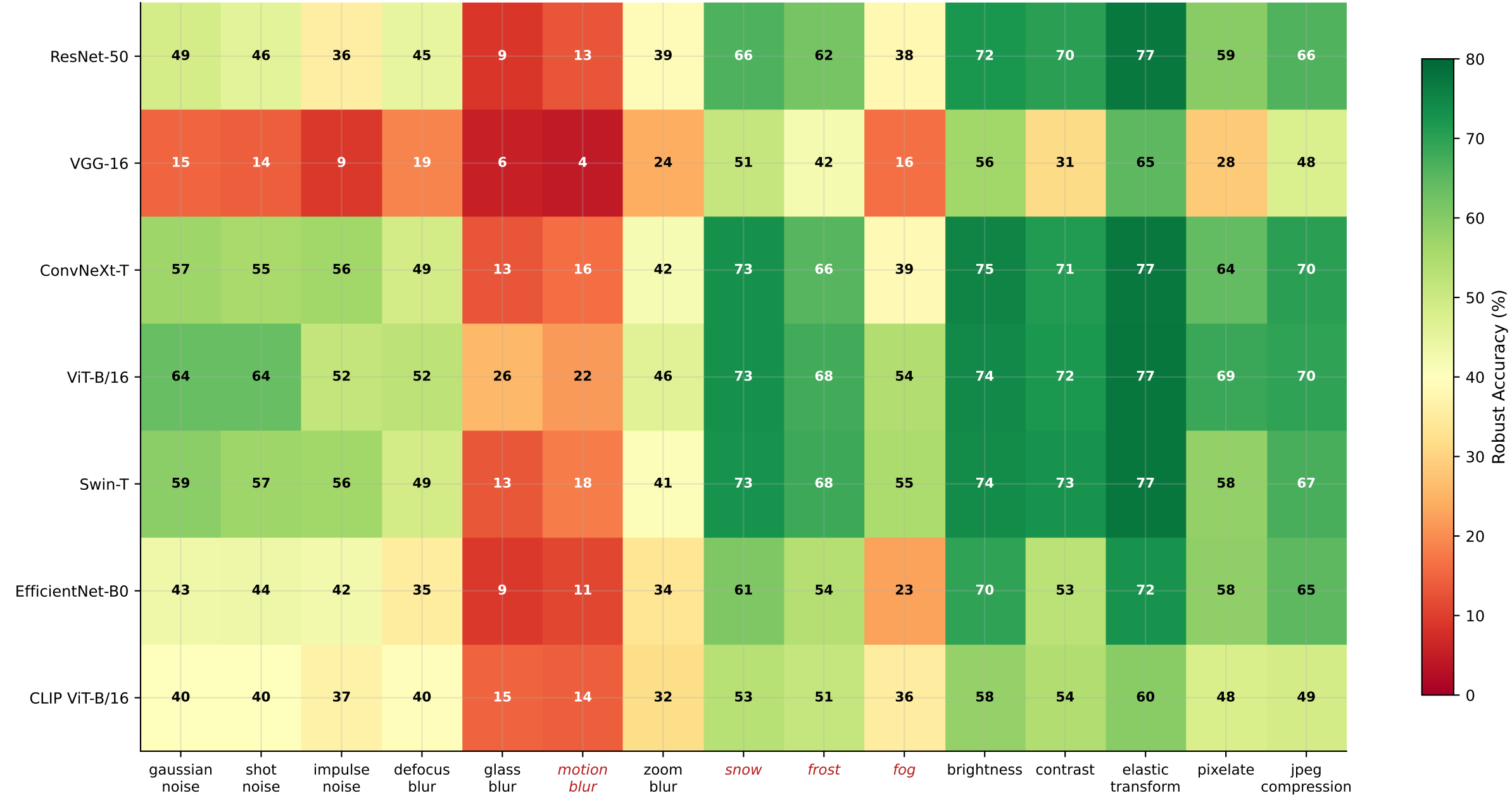
Axis 4 — ImageNet-C-style Corruptions: Robust Accuracy (%), severity 3 green = robust, red = fragile · italic columns = NumPy approximations
