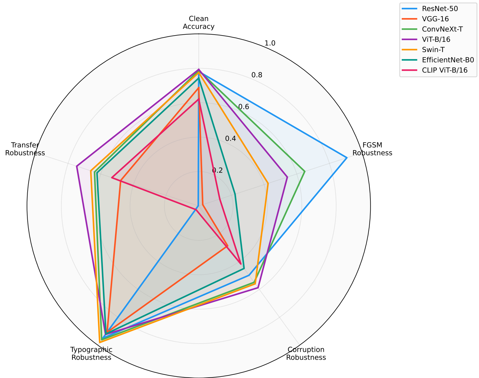
Robustness Radar — 7 Baselines (higher = better) PGD/AutoAttack omitted: all models ≈ 0 there
