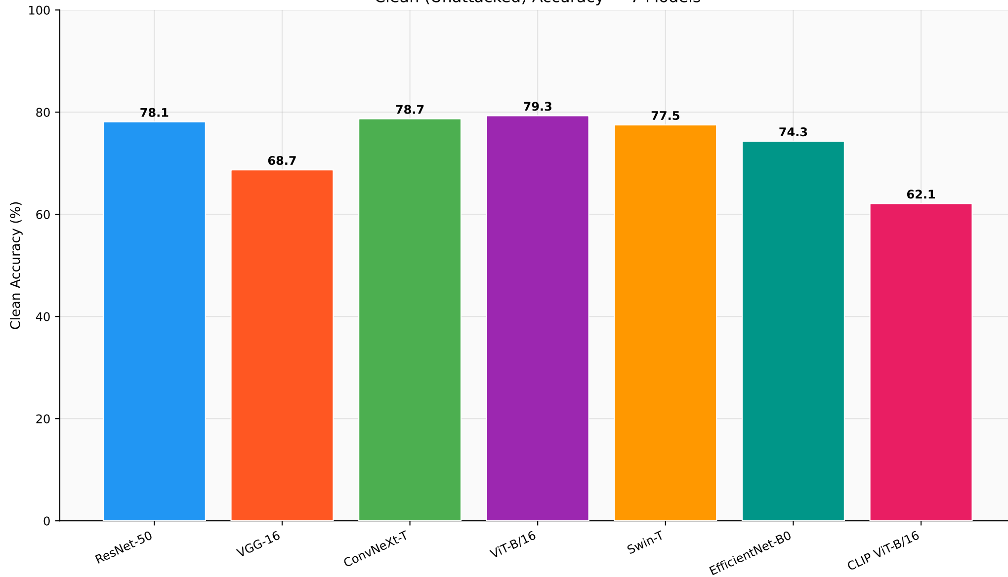
Clean (Unattacked) Accuracy — 7 Models
