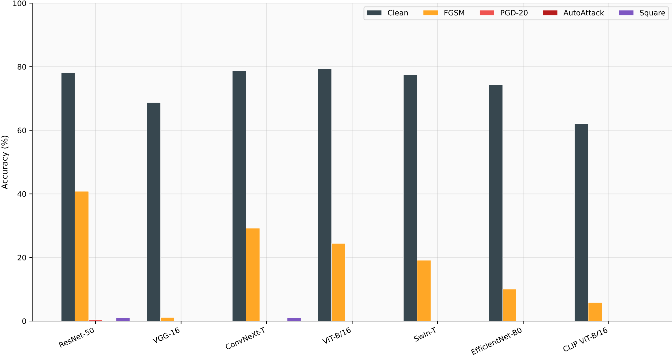
Axis 1 — Gradient Attacks per Model PGD/AutoAttack/Square drive every model to ~0% (no gradient masking)
