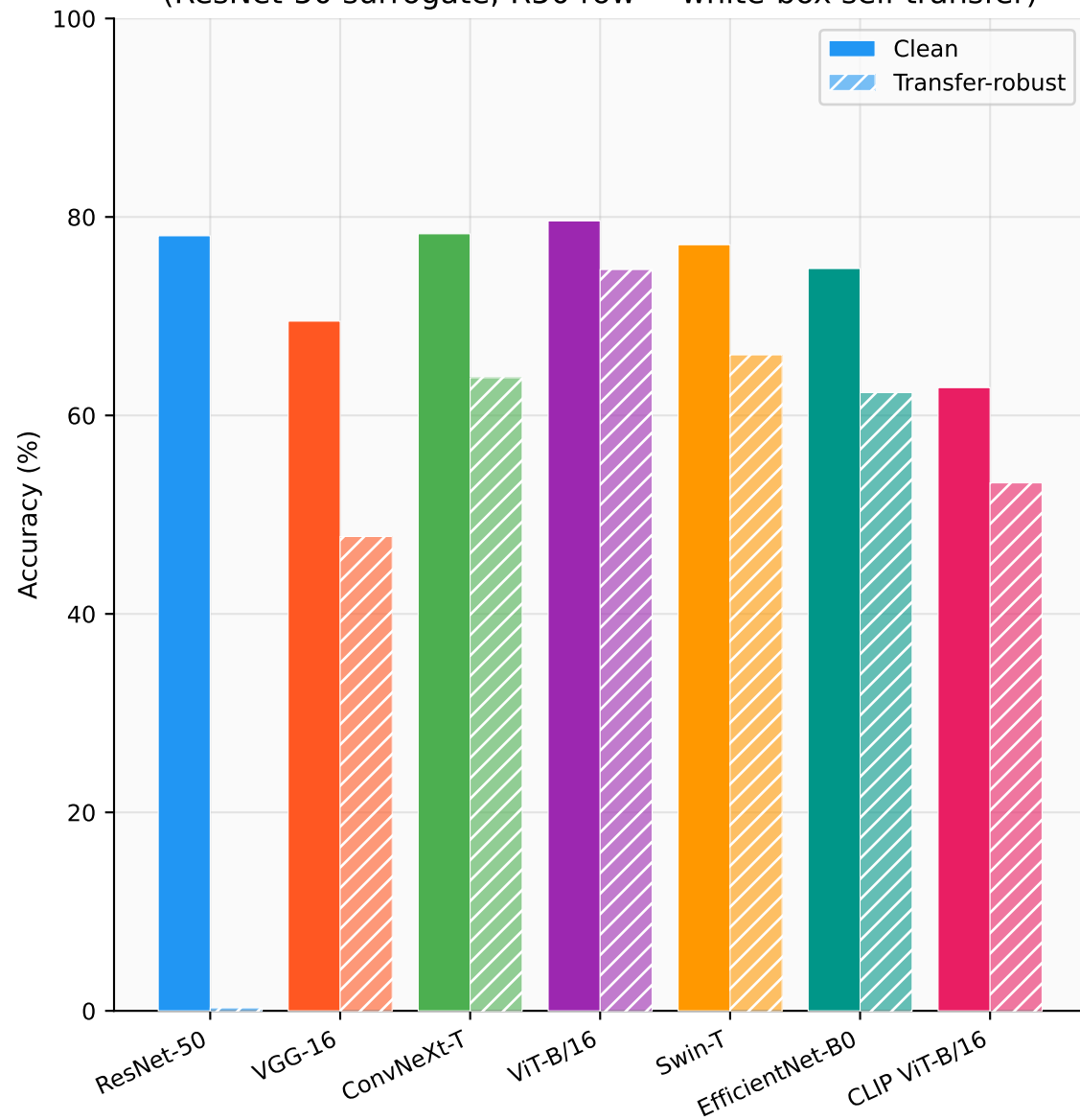
Axis 2 — Clean vs Transfer-Robust (ResNet-50 surrogate; R50 row = white-box self-transfer)
