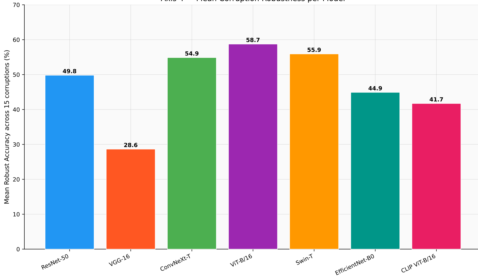
Axis 4 — Mean Corruption Robustness per Model
