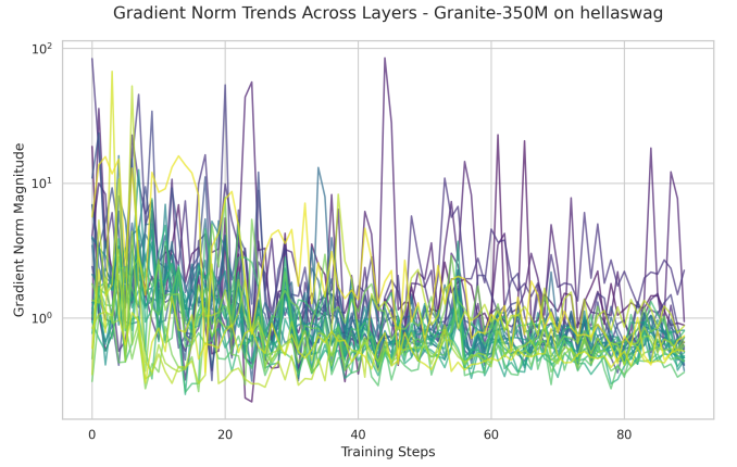
(b) Granite-350M on HellaSwag
