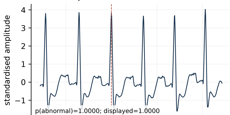
AFib label / AFib prediction record 201, 1597.602 s
