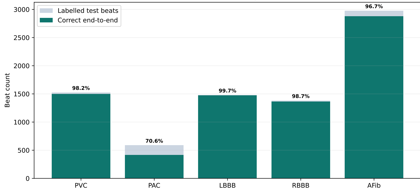
Final model: fixed 20% temporal holdout
