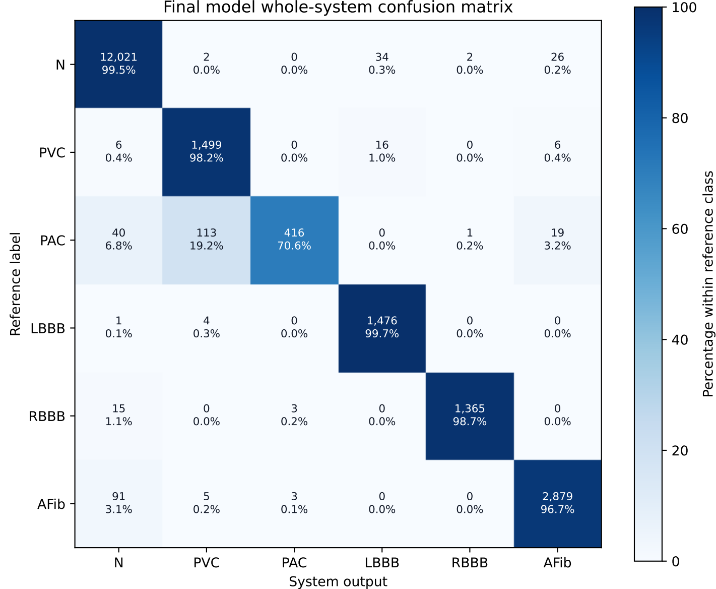
Final model whole-system confusion matrix
