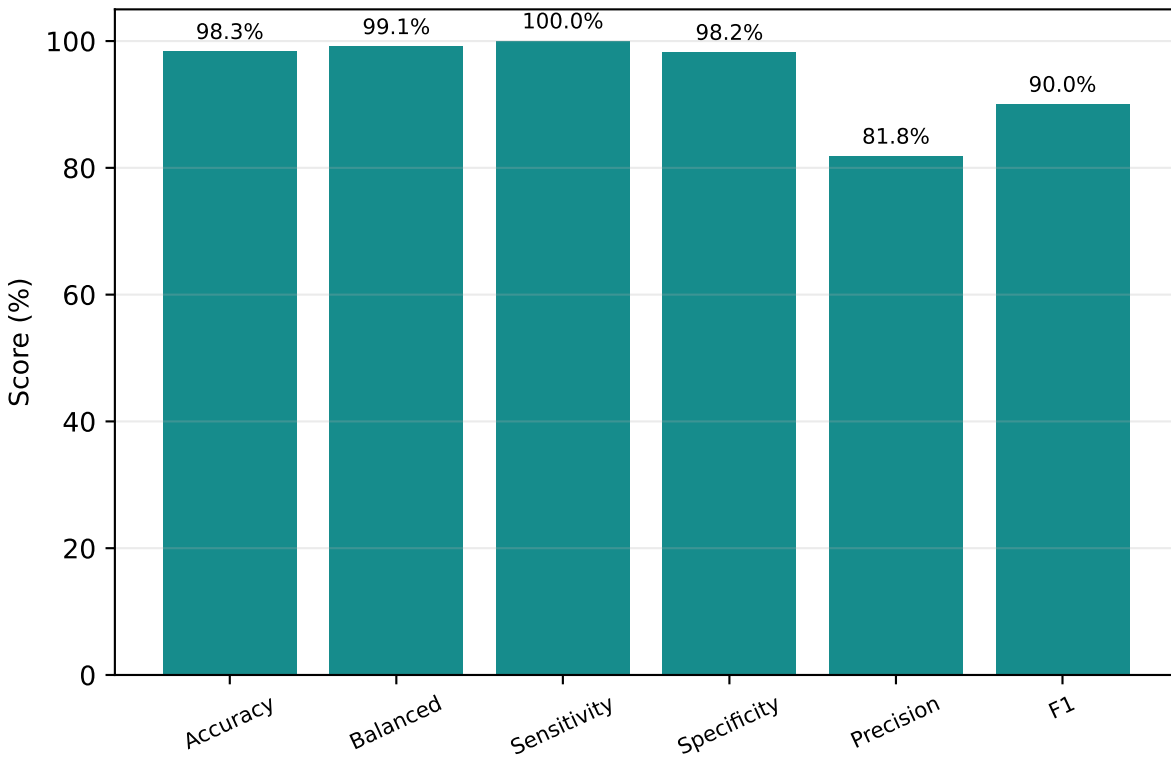
INCART external-check metrics
