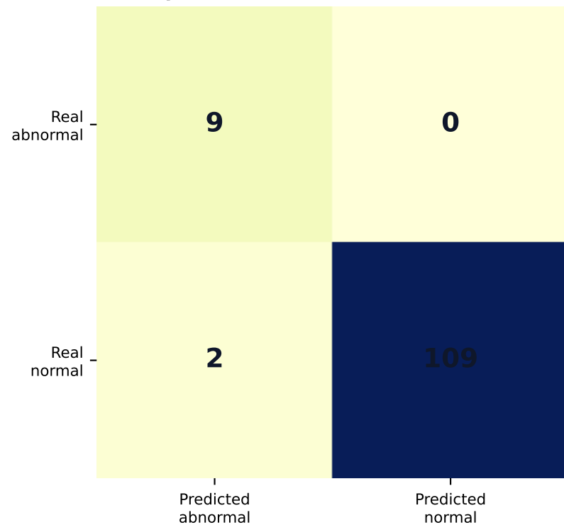
Binary confusion
