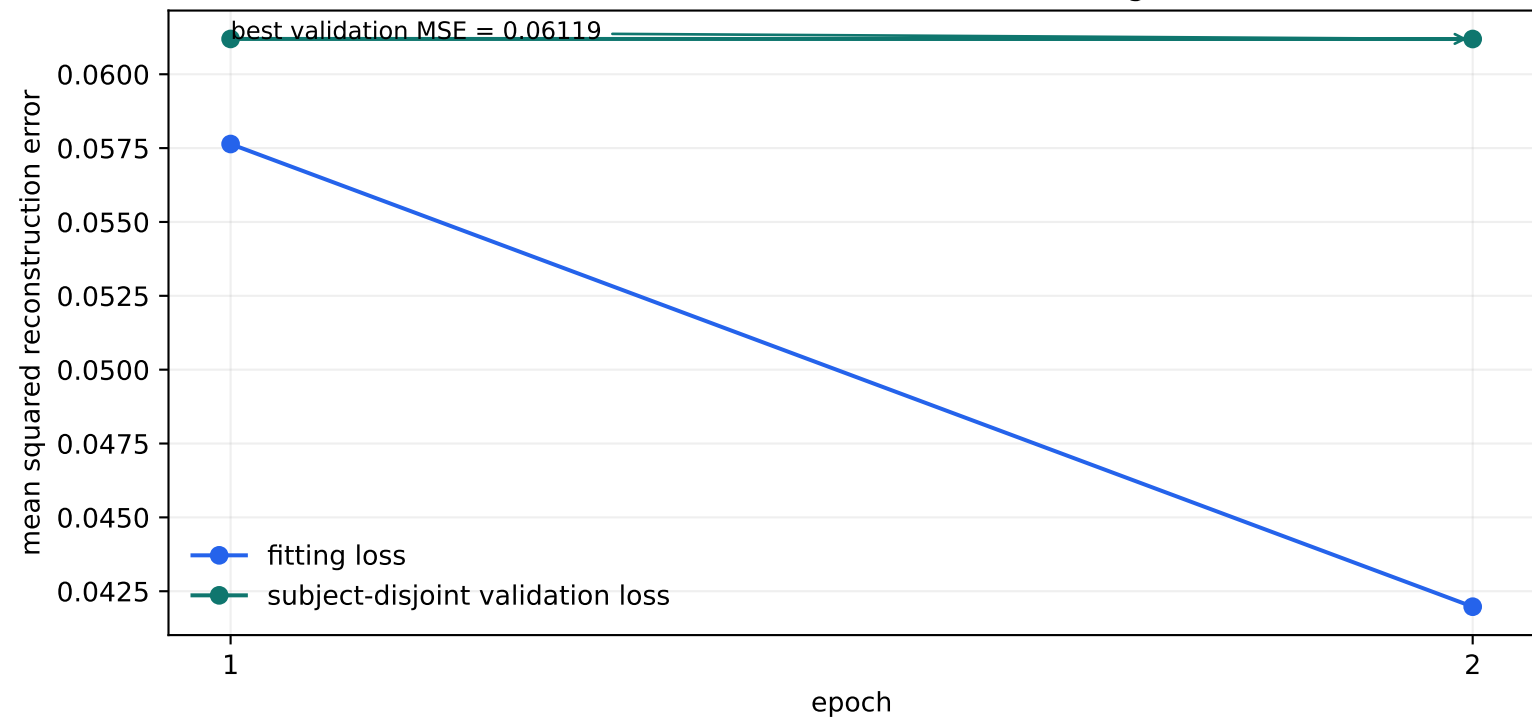
MIT-BIH normal-sinus autoencoder learning curve
