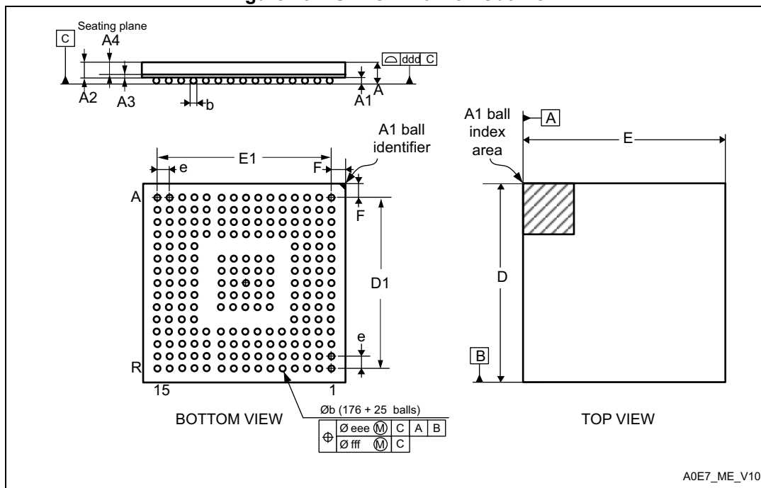
Figure 137. UFBGA176+25 - Outline
