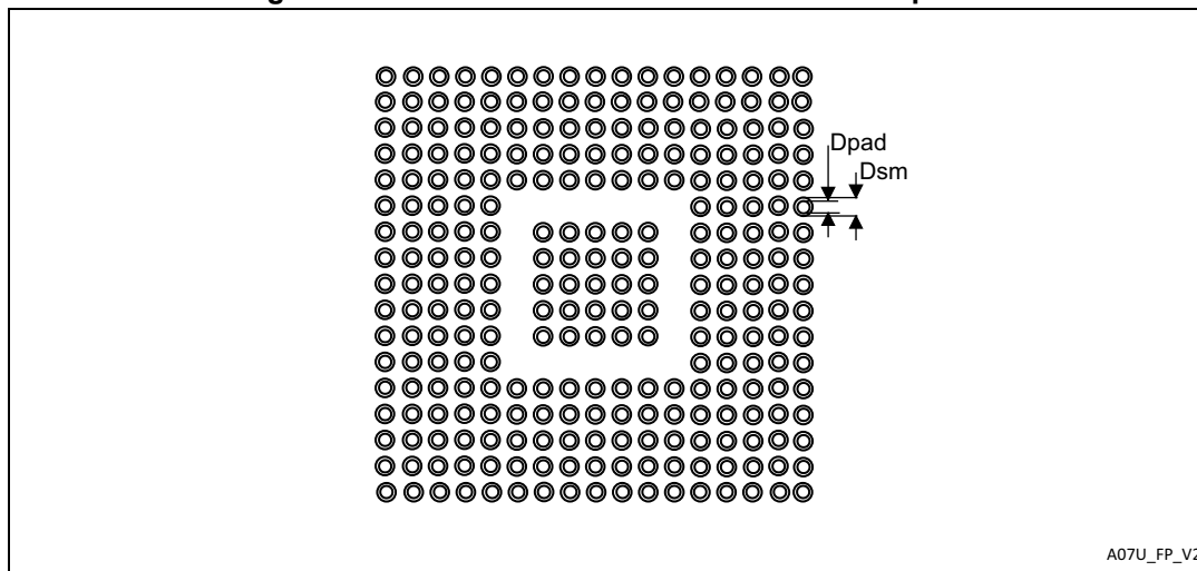
Figure 141. TFBGA240+25 - Recommended footprint
