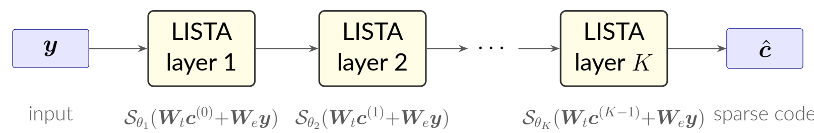
Figure 2. K -layer LISTA with tied weights \mathbf{W}_e, \mathbf{W}_t and per-layer learnable thresholds \theta_k . Each block is one ISTA-style update followed by soft-thresholding; the recurrence reproduces ISTA at initialisation.
