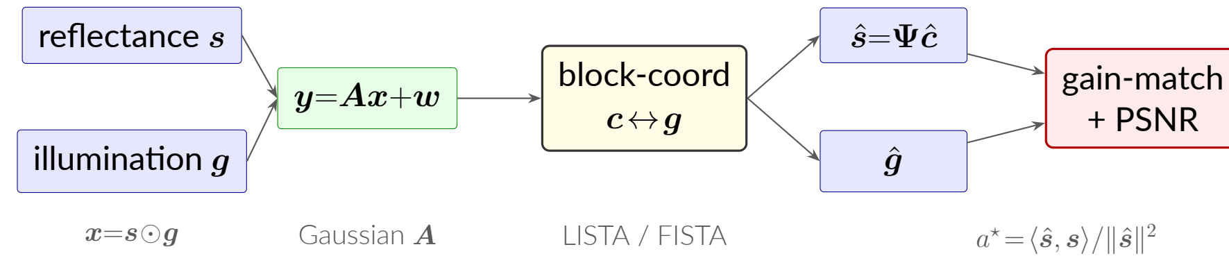
Figure 1. End-to-end joint recovery pipeline. The RAW signal \mathbf{x}=\mathbf{s}\odot\mathbf{g} is measured via Gaussian \mathbf{A} ; block-coordinate alternation recovers (\mathbf{c}, \mathbf{g}) simultaneously; the scalar gain ambiguity is resolved at evaluation.
