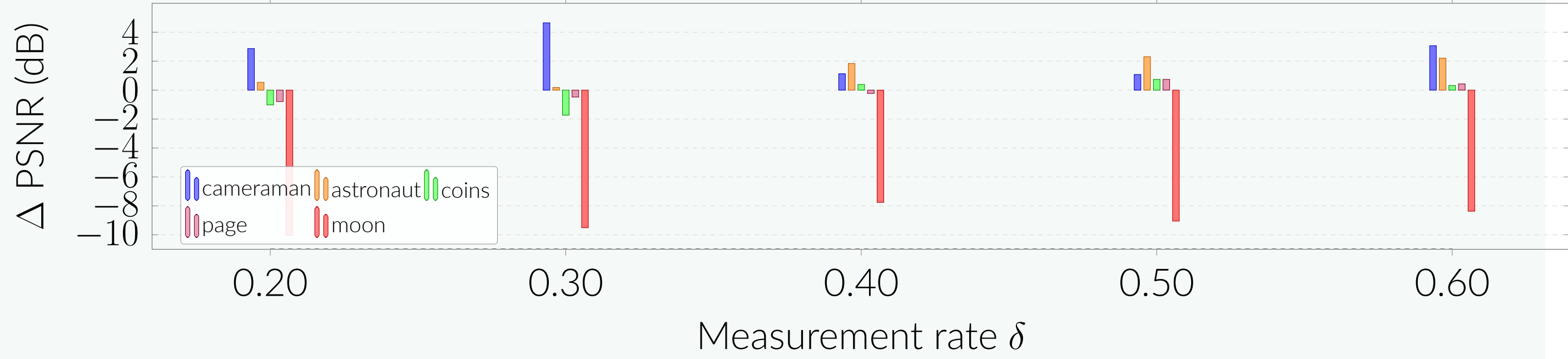
Figure 3. Per-scene PSNR gain over the sequential baseline. Textured wins +1.1 to +4.7 dB on cameraman, astronaut; moon collapses by \sim 8 dB – a real, mechanism-explainable failure mode.
