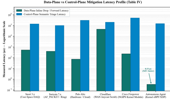
Fig. 4. Log-scale latency spectrum comparing data-plane mitigation and control-plane triage (Table IV).
