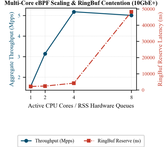
FIGURE 9. Empirical multi-core eBPF scaling and lock-free ring-buffer reservation latency under 10GbE-oriented workload emulation (software packet-processing emulation on physical CPU cores; not a physical 10GbE NIC measurement) across K \in \{1, 2, 4, 8\} physical cores. Linear scaling is achieved across 1–4 cores, while atomic reservation contention on a monolithic ring buffer emerges at 8 cores, motivating per-queue partitioned buffers.
