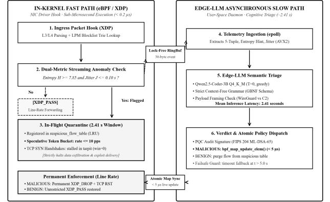
FIGURE 2. Dual-Horizon asynchronous triage and in-flight fast-path packet filtering lifecycle during the Edge-LLM's 2.41 s reasoning window. In-kernel eBPF clamps suspicious flows to a speculative token-bucket rate limiter (10 pps) or zero-window tarpit while the user-space Edge-LLM deliberates asynchronously, preventing data exfiltration before atomic kernel rule enforcement ( < 5 \mu\text{s} ).
