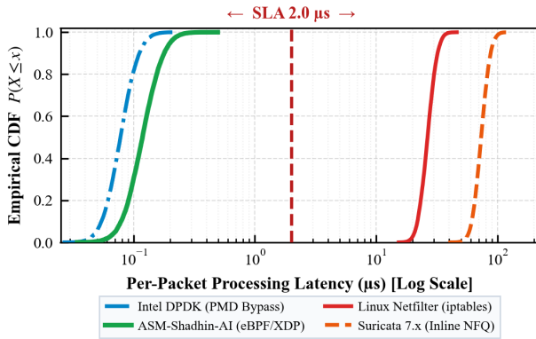
FIGURE 7. Empirical cumulative distribution function (CDF) of per-packet processing latency ( \mu s) pooled across N = 30 independent benchmark trials. Both ASM-Shadhin-AI (0.126 \mu s mean) and DPDK (0.081 \mu s mean) remain well within a 2.0 \mu s high-rate service level target; Netfilter and Suricata exceed 10 \mu s at the median. Latency values from bpf_ktime_get_ns() .
