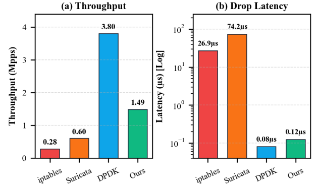
FIGURE 5. Architectural performance comparison across four systems on identical hardware (Intel i5-4570, N = 30 trials, mean \pm s.d.): (a) packet throughput in Mpps and (b) mean per-packet processing latency in \mu\text{s} (log scale). ASM-Shadhin-AI achieves 1.495 Mpps at 0.126 \mu\text{s} mean latency. DPDK achieves higher raw throughput (3.798 Mpps, 0.081 \mu\text{s} ) under dedicated PMD core polling.
