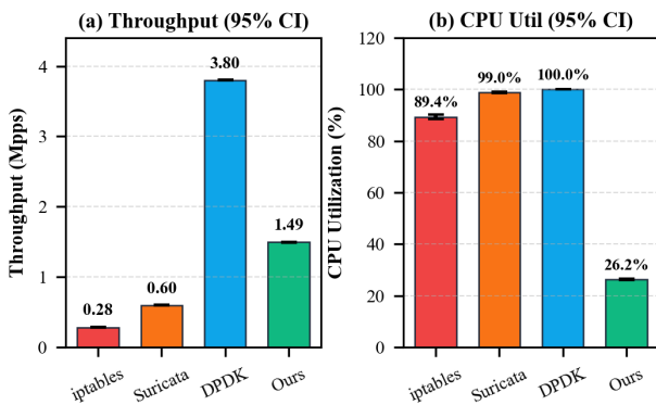
FIGURE 8. 95% confidence intervals for mean throughput (Mpps) and mean CPU utilization (%) across N = 30 repeated benchmark runs on identical hardware, computed using Welch-Satterthwaite t -based intervals ( \alpha = 0.05 ). ASM-Shadhin-AI 95% CI: throughput [1.489, 1.500] Mpps, CPU [25.8, 26.6]%.
