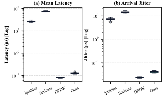
FIGURE 6. Boxplots of per-packet processing latency ( \mu\text{s} , log scale) across N = 30 independent benchmark trials. Each trial uses an identical 10,000,000-packet PCAP corpus replayed at the generator's top-speed setting with full driver, NIC ring, and CPU state resets between runs. Boxes span the interquartile range; whiskers extend to 1.5\times IQR. Latency reported is the in-kernel measurement via bpf_ktime_get_ns() .
