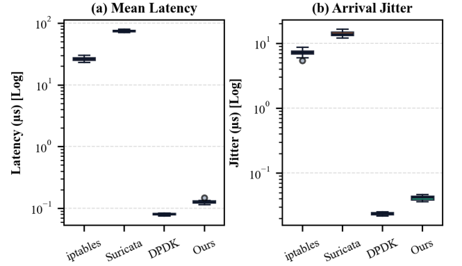
Fig. 6. Boxplots of per-packet processing latency ( \mu\text{s} , log scale) across N = 30 independent benchmark trials. Each trial uses an identical 10,000,000-packet PCAP corpus replayed at the generator’s top-speed setting with full driver, NIC ring, and CPU state resets between runs. Boxes span the interquartile range; whiskers extend to 1.5\times\text{IQR} . Latency reported is the in-kernel measurement via bpf_ktime_get_ns() .
