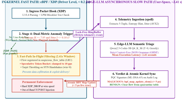
Fig. 2. Dual-Horizon asynchronous triage and in-flight fast-path packet filtering lifecycle during the Edge-LLM’s 2.41s reasoning window. In-kernel eBPF clamps suspicious flows to a speculative token-bucket rate limiter (10 pps) or zero-window tarpit while the user-space Edge-LLM deliberates asynchronously, preventing data exfiltration before atomic kernel rule enforcement ( < 5 \mu\text{s} ).
