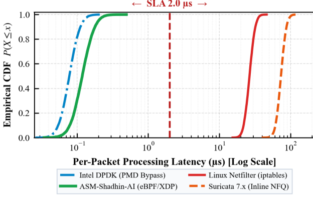
Fig. 6. Empirical cumulative distribution function (CDF) of per-packet processing latency ( \mu s) pooled across N = 30 independent benchmark trials. Both ASM-Shadhin-AI ( 0.126 \mu s mean) and DPDK ( 0.081 \mu s mean) remain well within a 2.0 \mu s line-rate service level target; Netfilter and Suricata exceed 10 \mu s at the median. Latency values from bpf_ktime_get_ns() .
