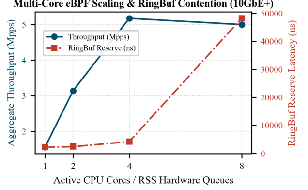
Fig. 9. Empirical multi-core eBPF scaling and lock-free ring-buffer reservation latency under 10GbE+ line-rate burst emulation across K \in \{1, 2, 4, 8\} physical cores. Linear scaling is achieved across 1–4 cores, while atomic reservation contention on a monolithic ring buffer emerges at 8 cores, motivating per-queue partitioned buffers.
