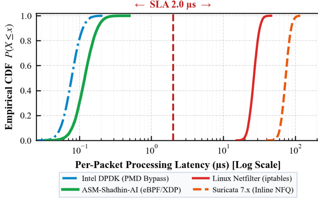
Fig. 7. Empirical cumulative distribution function (CDF) of per-packet processing latency ( \mu\text{s} ) pooled across N = 30 independent benchmark trials. Both ASM-Shadhin-AI (0.126 \mu\text{s} mean) and DPDK (0.081 \mu\text{s} mean) remain well within a 2.0 \mu\text{s} line-rate service level target; Netfilter and Suricata exceed 10 \mu\text{s} at the median. Latency values from bpf_ktime_get_ns() .
