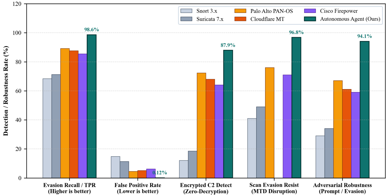
FIG. 3. Detection accuracy and evasion resistance comparison across 10M flows (Table III).
