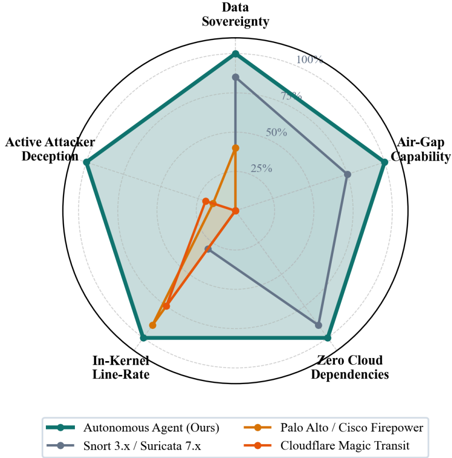
FIG. 2. Architectural sovereignty, air-gap capability, and autonomy comparison.
