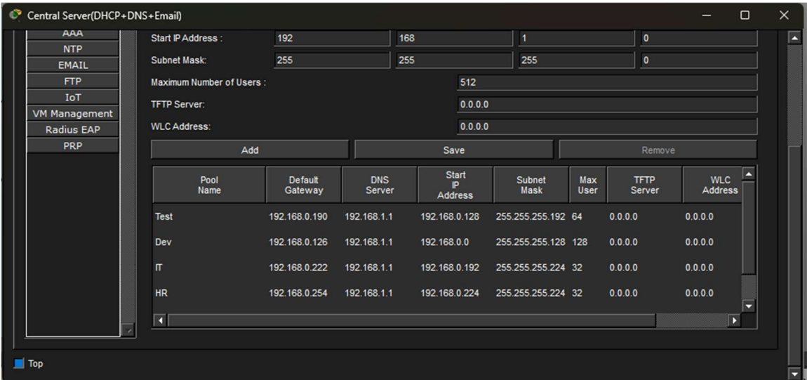
Fig4. DHCP Configuration
