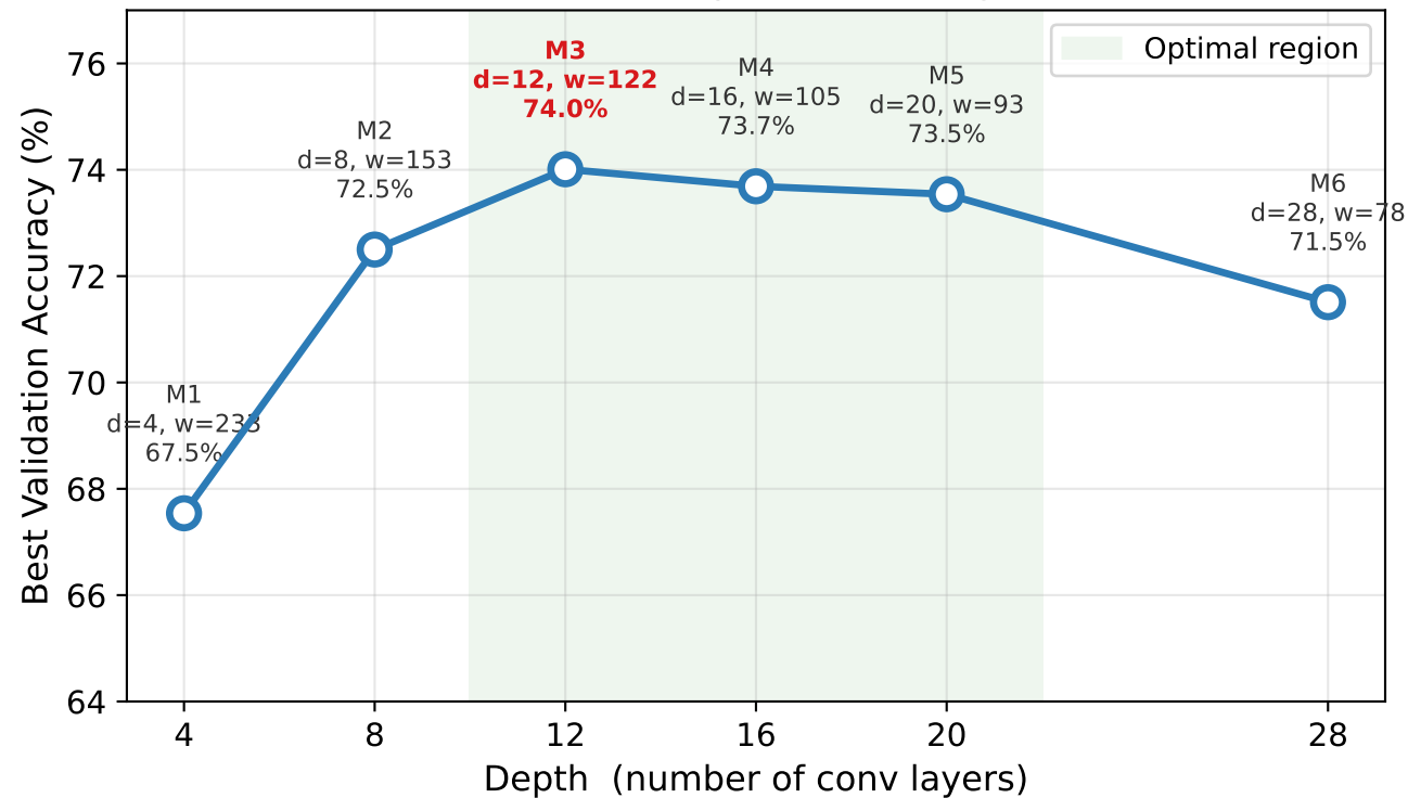
Depth-Width Trade-off on CIFAR-100 (fixed \sim 1.5 M parameter budget)
