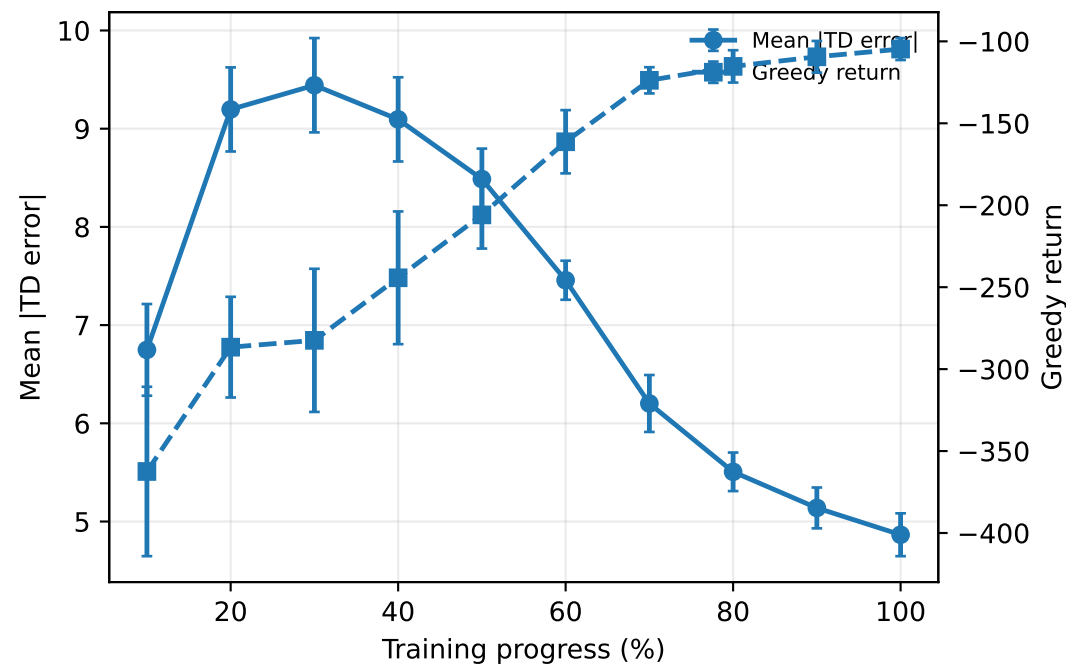
Acrobot
