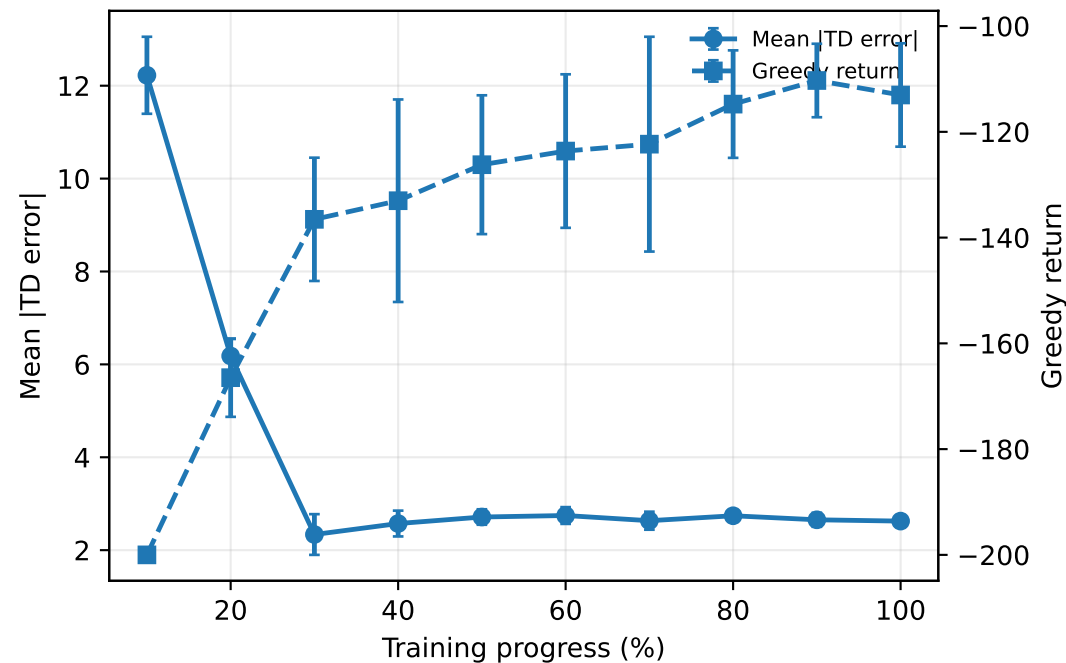
Acrobot
