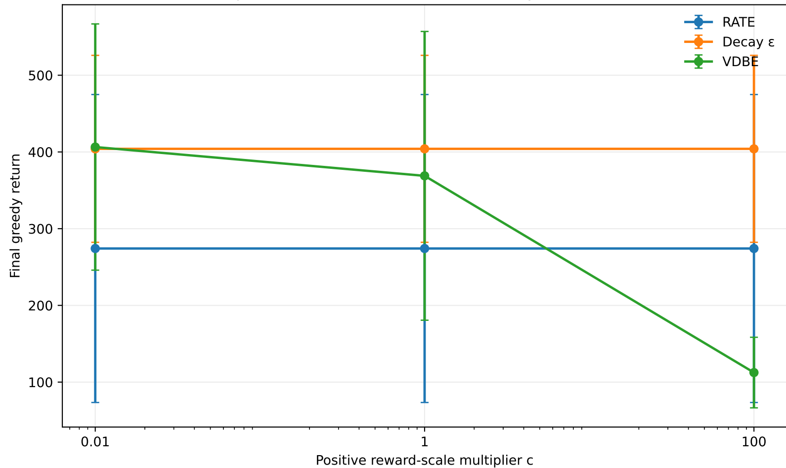
Experiment C — reward-scale sensitivity on CartPole
