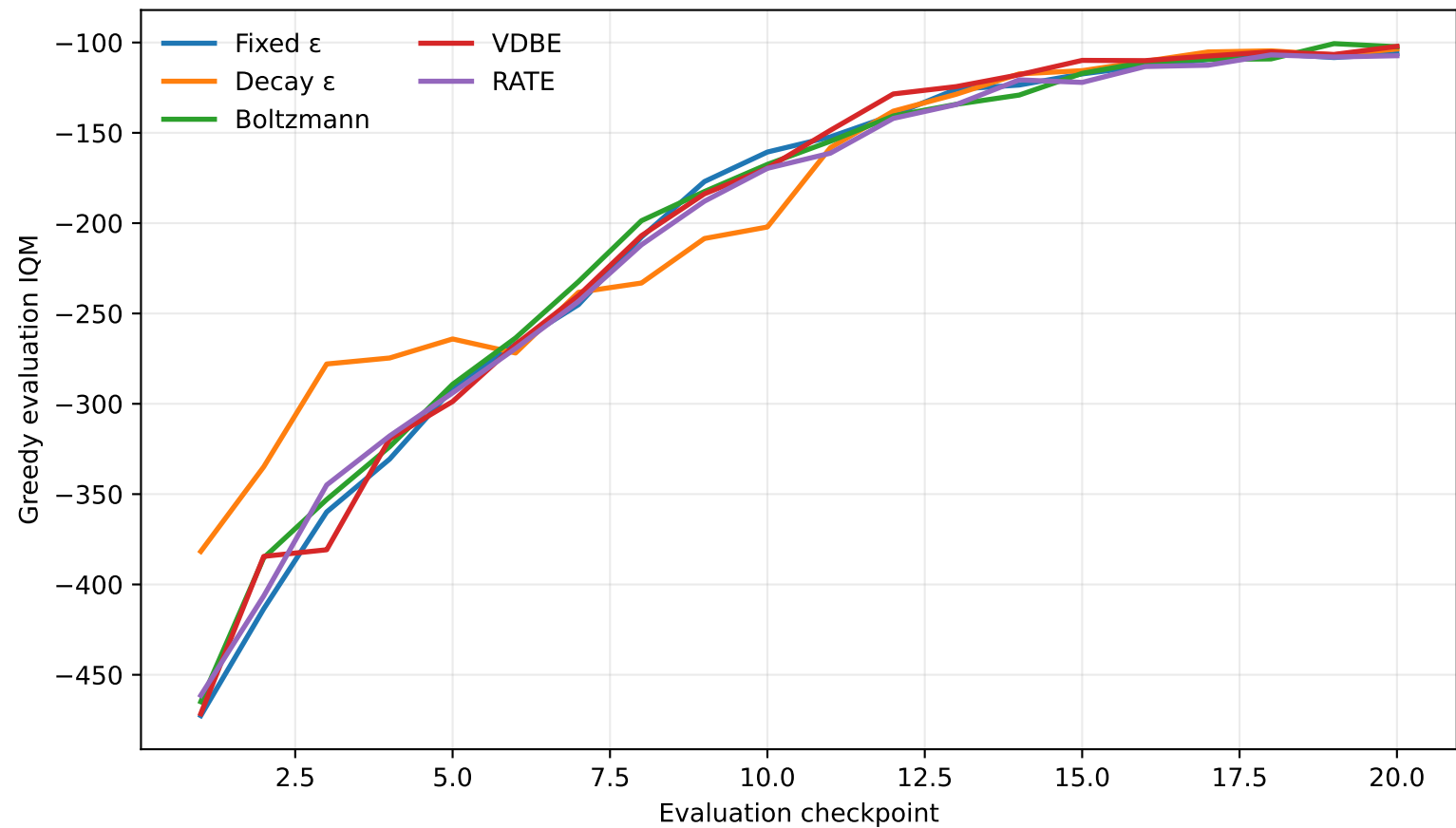
Acrobot — Linear Sarsa( \lambda )
