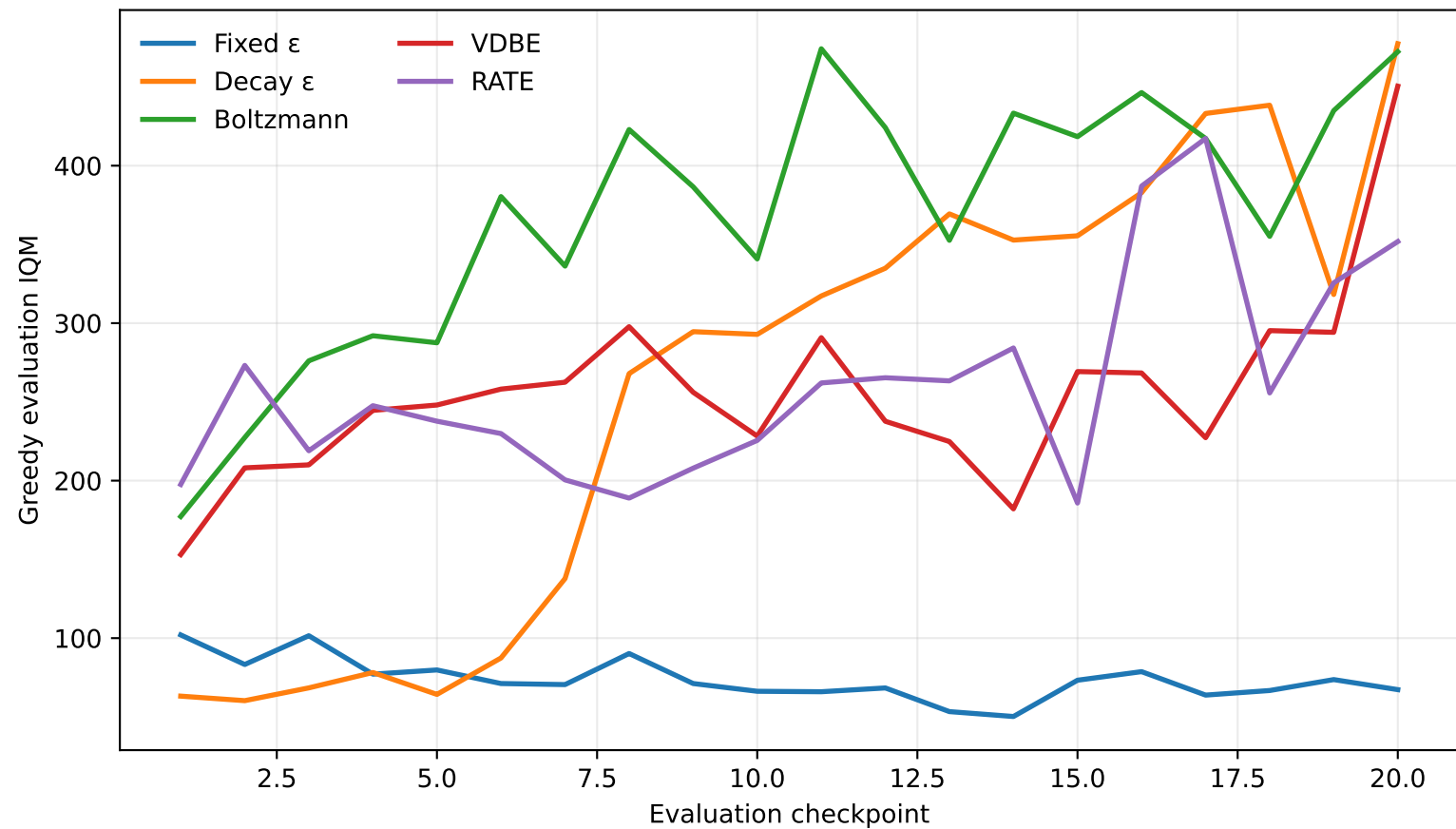
CartPole — Linear Sarsa( \lambda )
