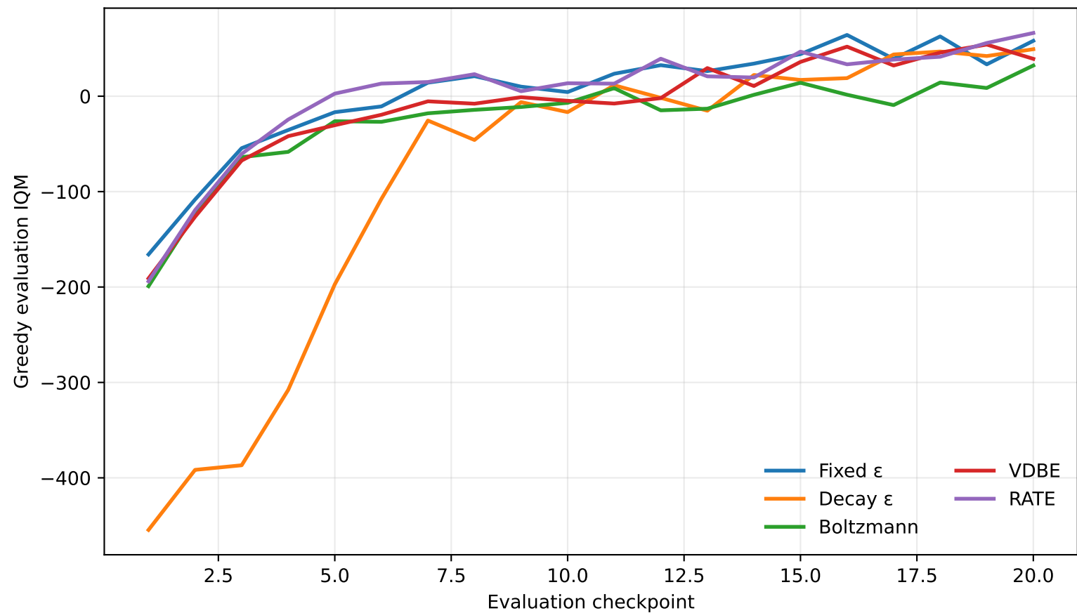
LunarLander — Linear Sarsa( \lambda )
