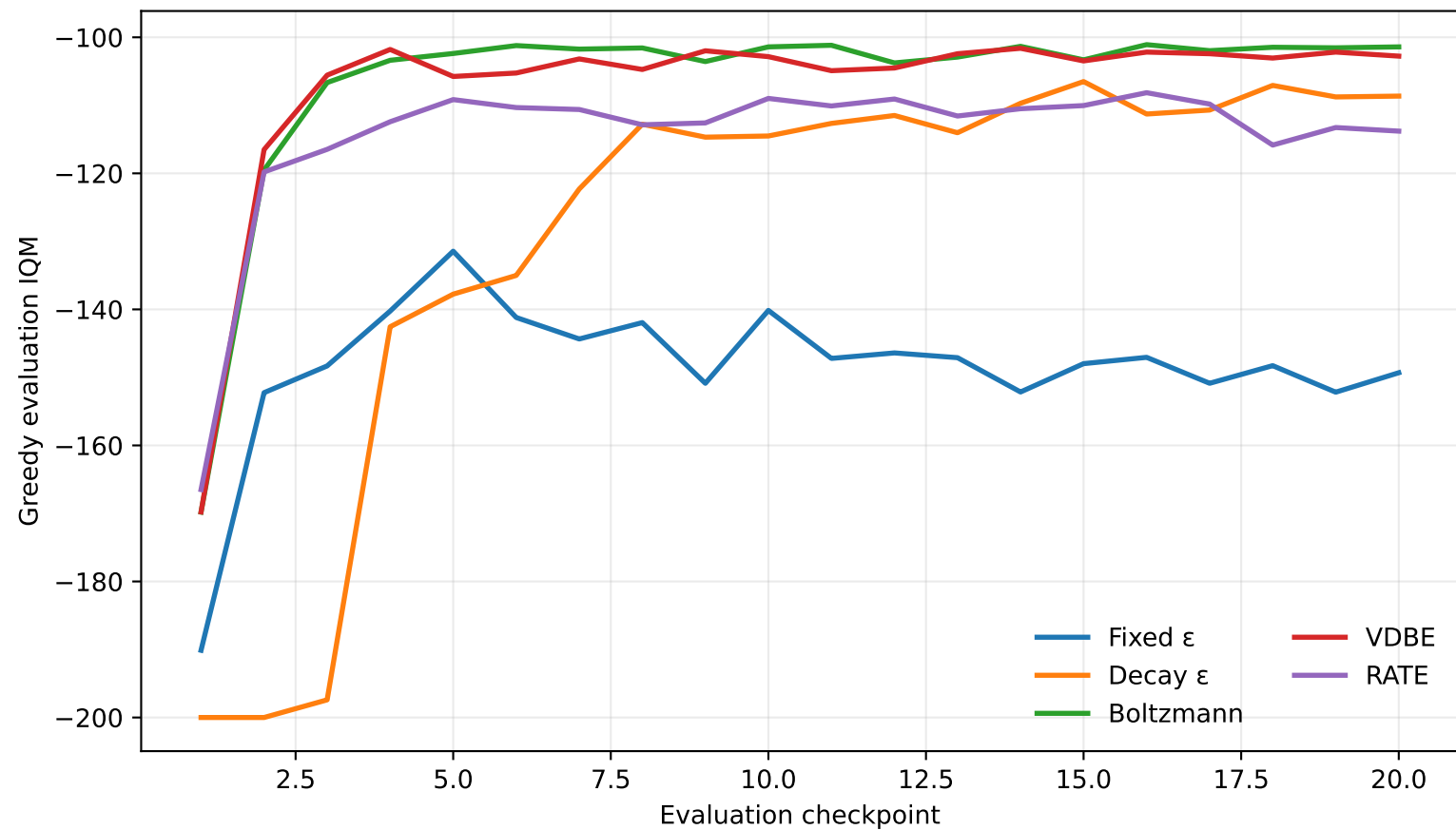
MountainCar — Linear Sarsa( \lambda )
