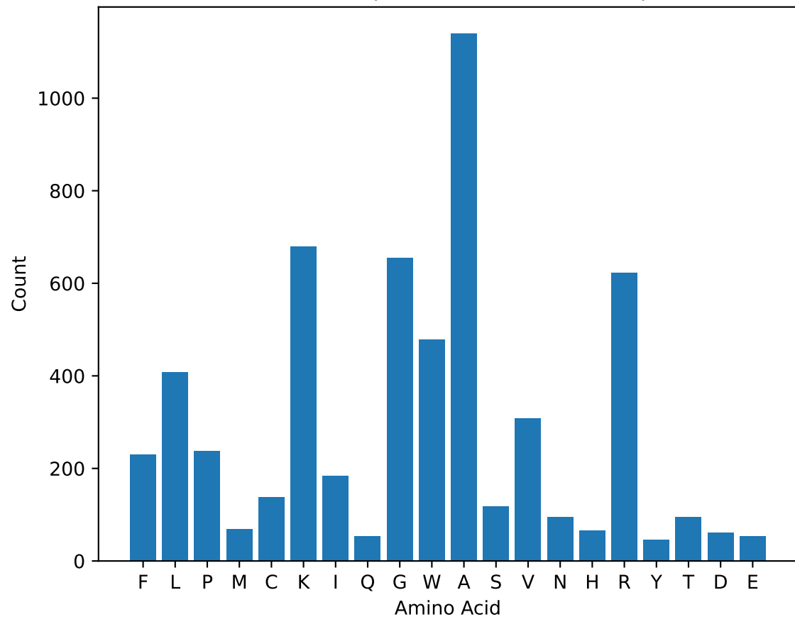
Amino Acid Composition - Generated Peptides
