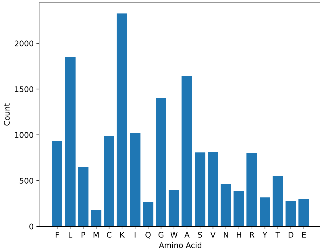
Amino Acid Composition - Real ACP
