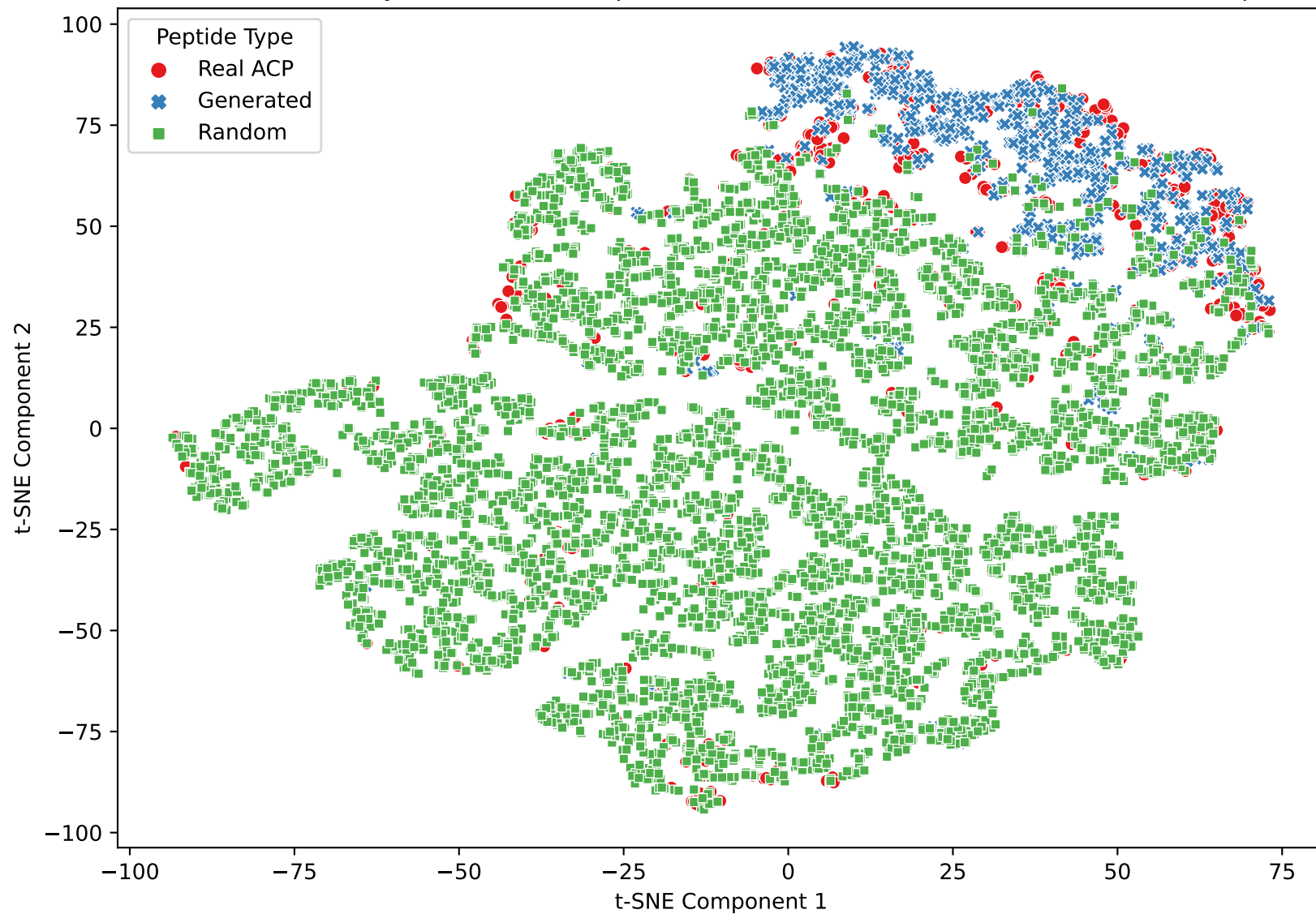
t-SNE Plot of the Physio-Chemical Properties of Real ACPs, Generated and Random Peptides
