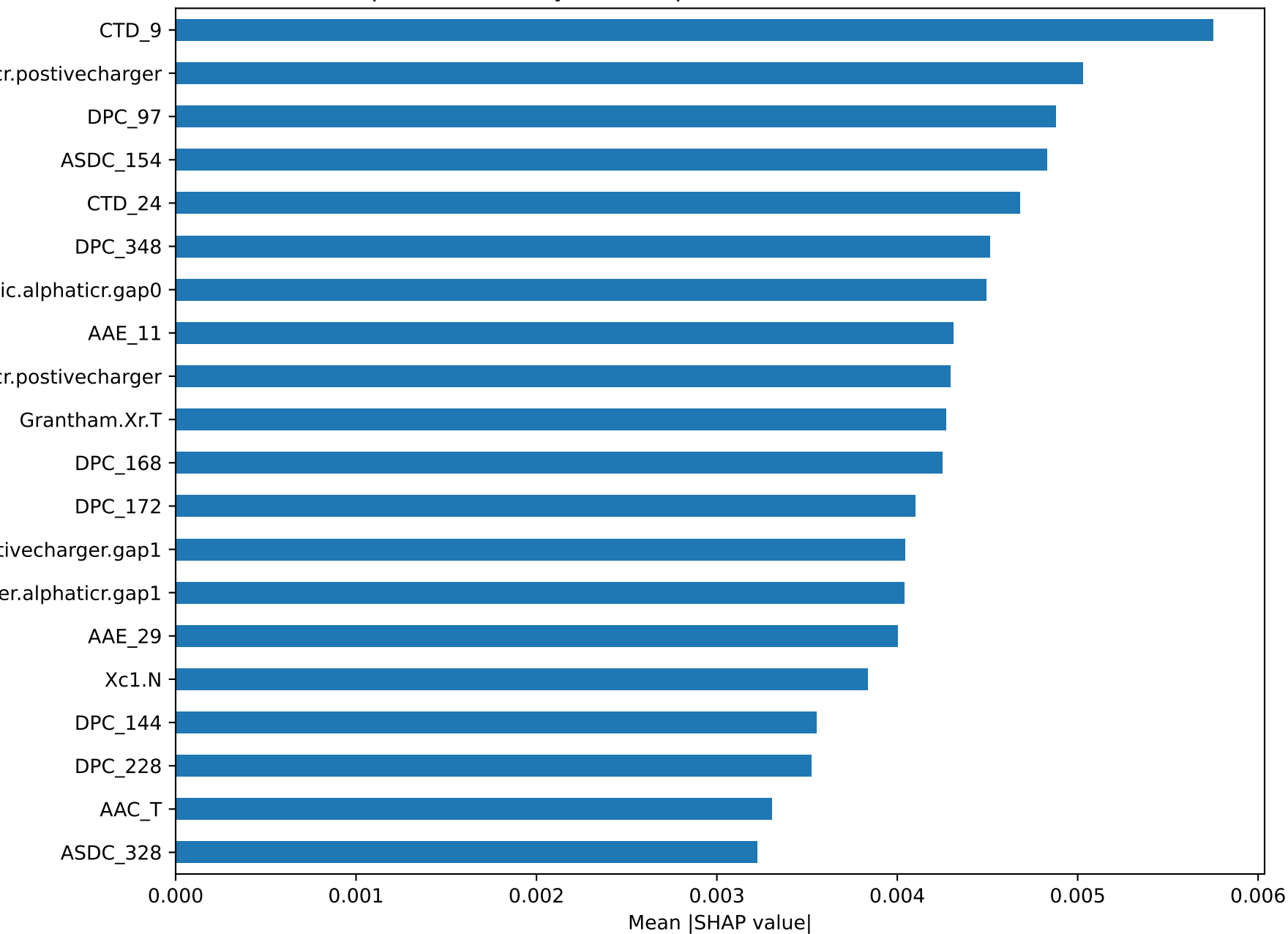
Top 20 Features by SHAP Importance for GAN-ML[Main Dataset]
