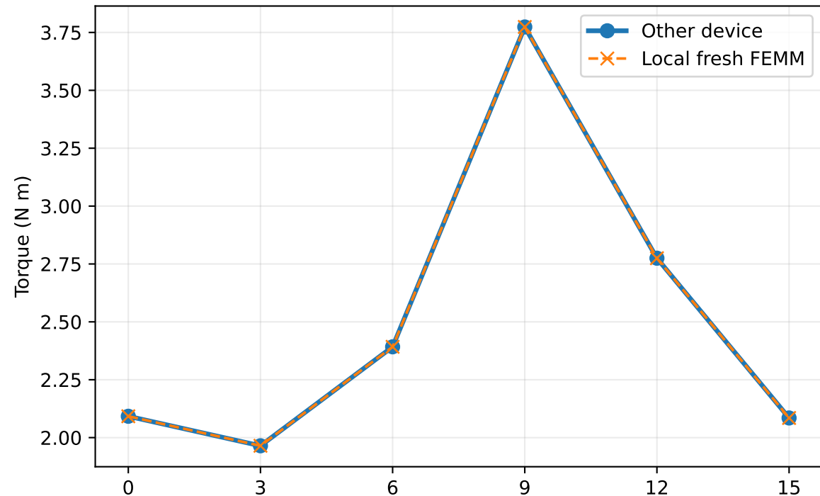
03 pilot cross-device check | 3.5 A, current phase = 4 x travel | Min Angle = 15 deg b31089763d90 | U | PM cells: 120
