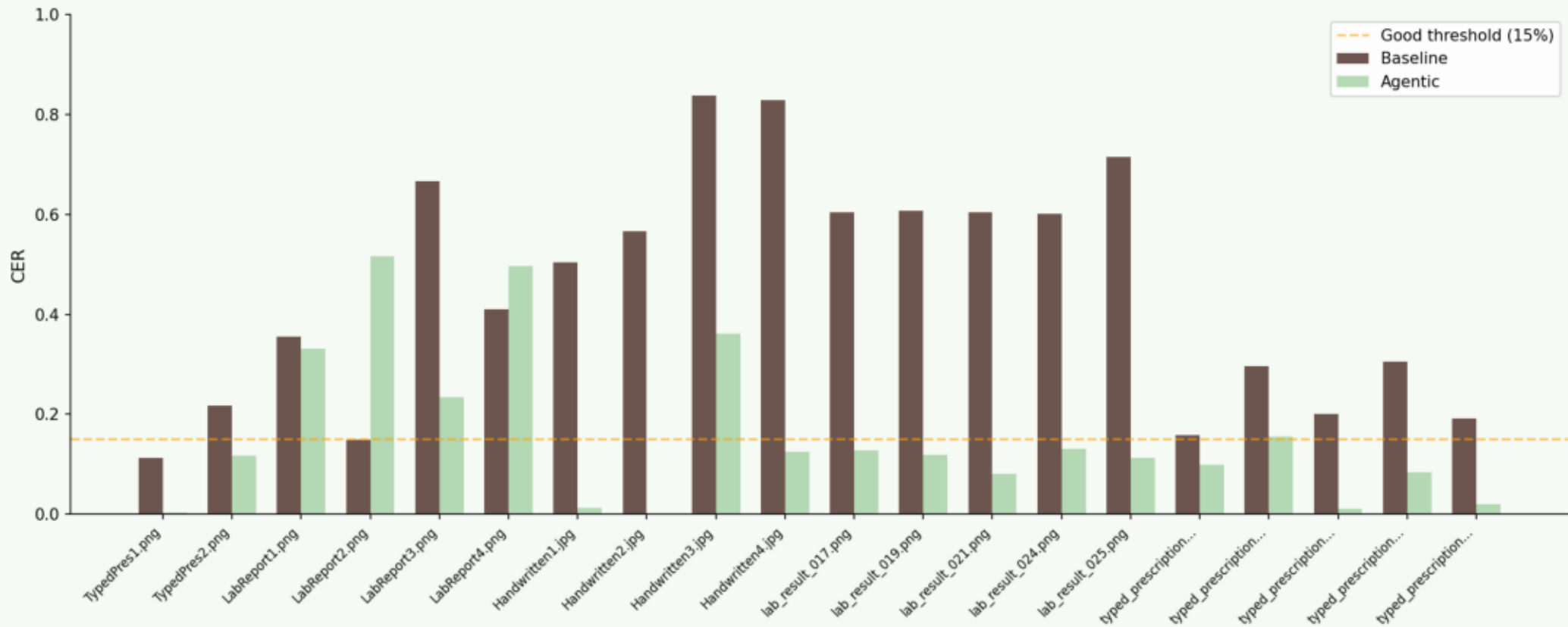
Character Error Rate (CER) Per Document
