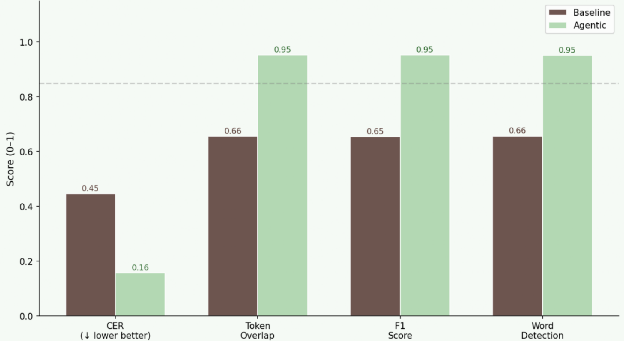
Overall Performance Comparison — Baseline vs Agentic
