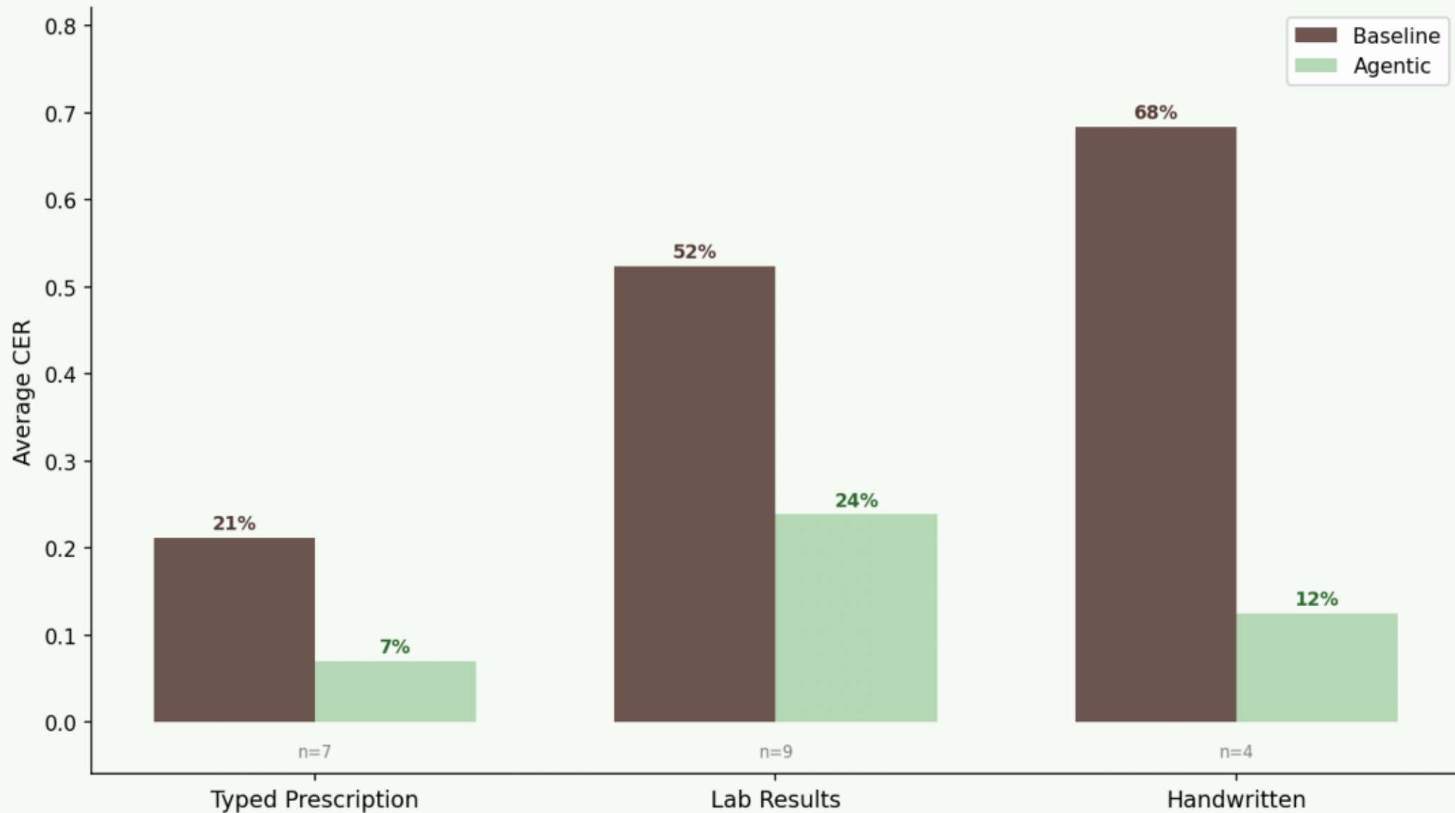
Average CER by Document Type
