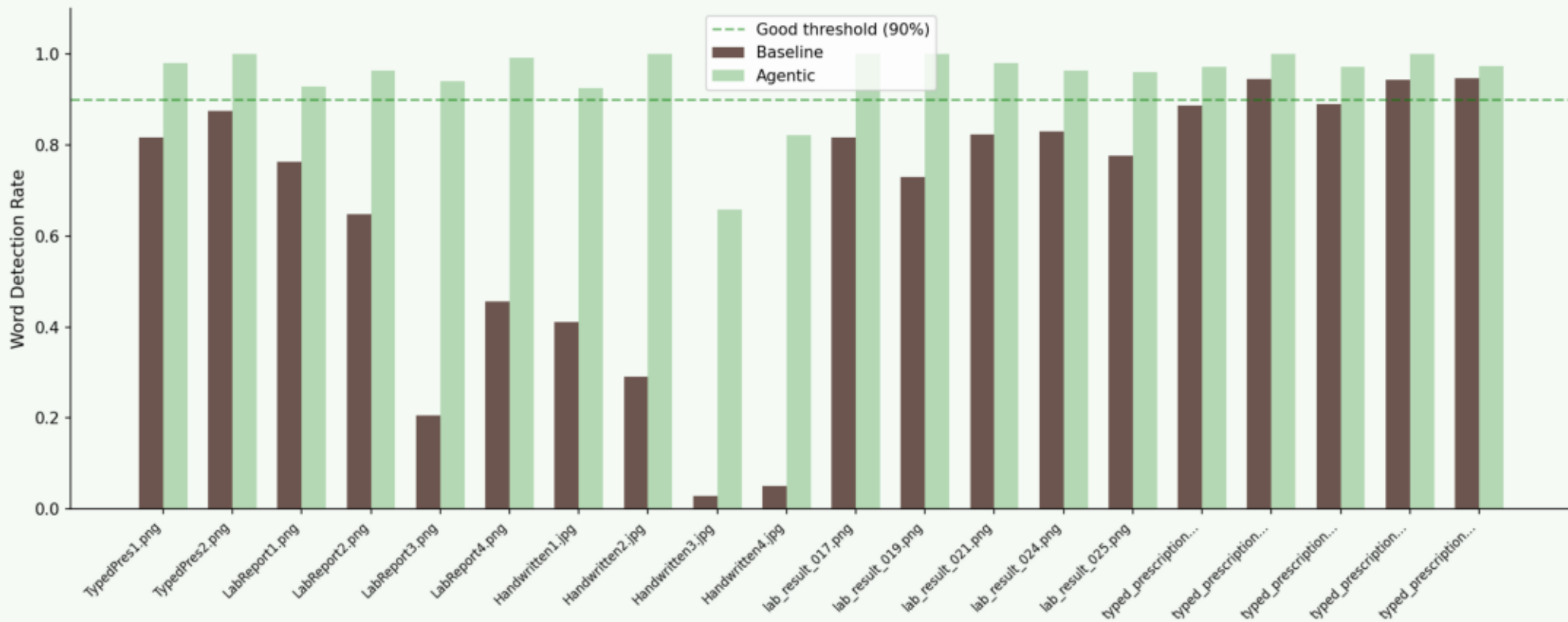
Word Detection Rate Per Document
