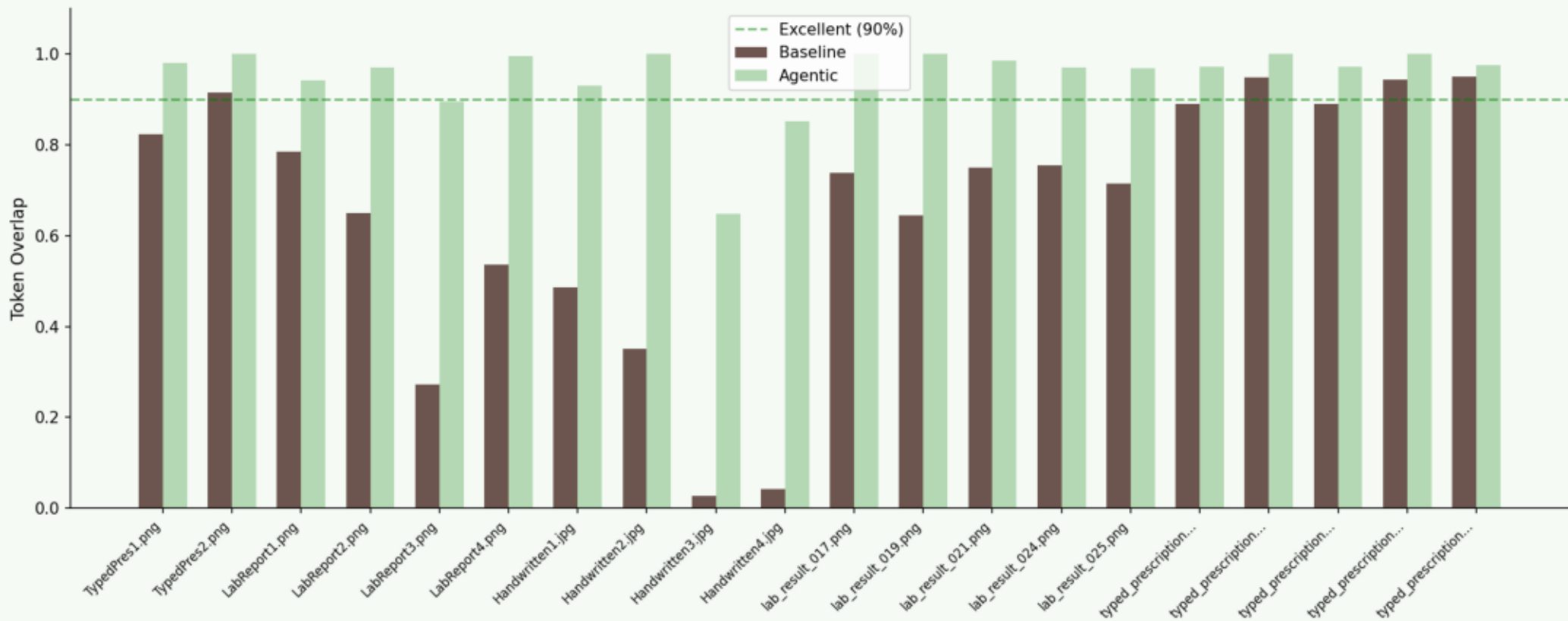
Token Overlap Per Document
