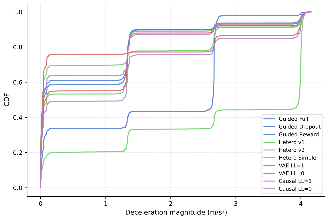
Deceleration CDF
