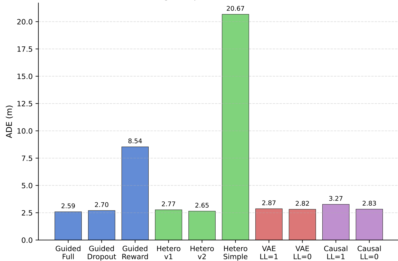
Average Displacement Error (ADE)
