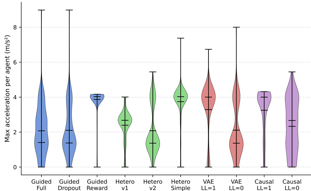
Maximum Acceleration per Agent
