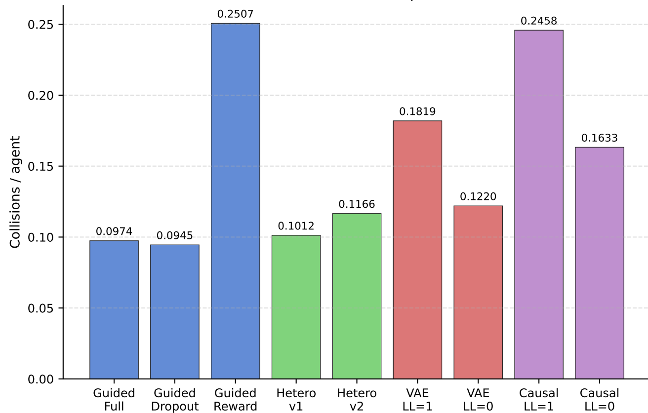
WOSAC Collision Rate (Simulated) [from WOSAC exp1]
