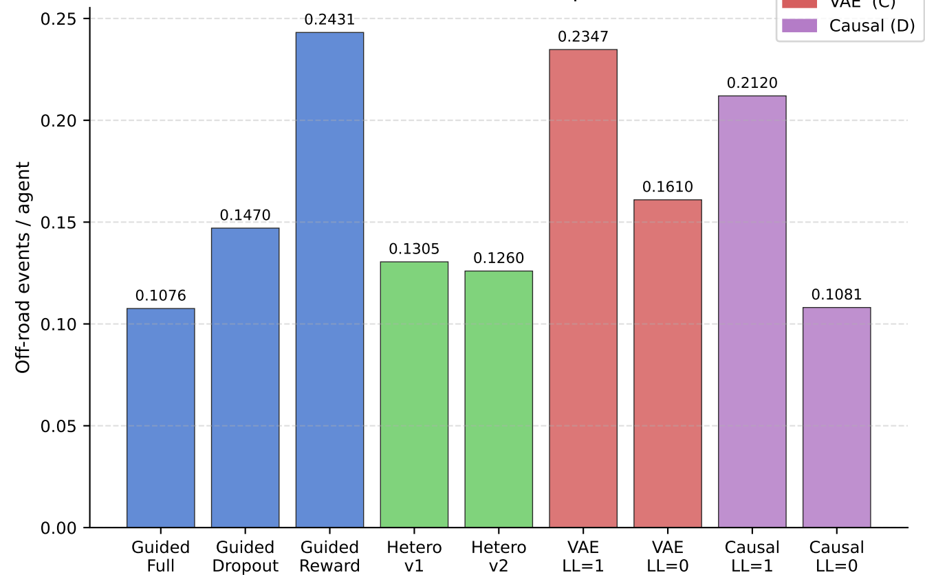
WOSAC Off-road Rate (Simulated) [from WOSAC exp1]
