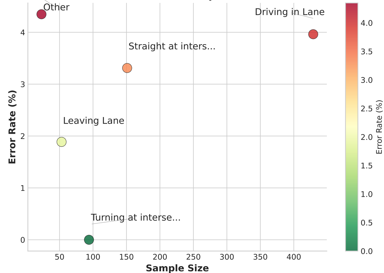
Error Rate vs Sample Size
