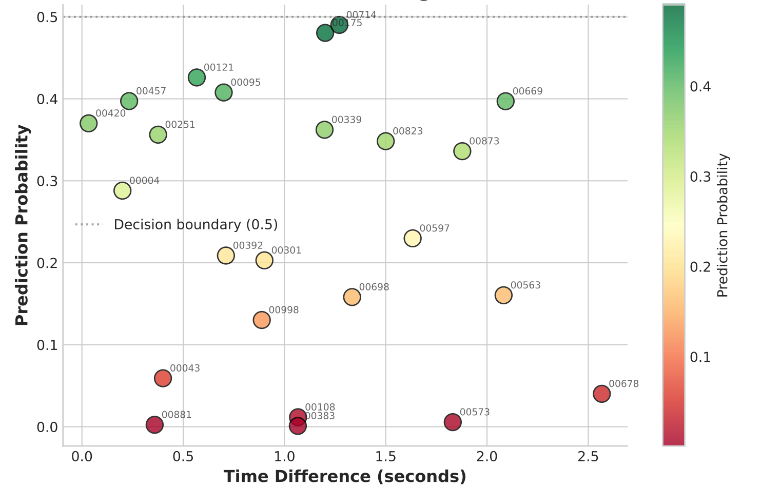
Time Difference vs Model Confidence (Red = confident wrong = BAD)
