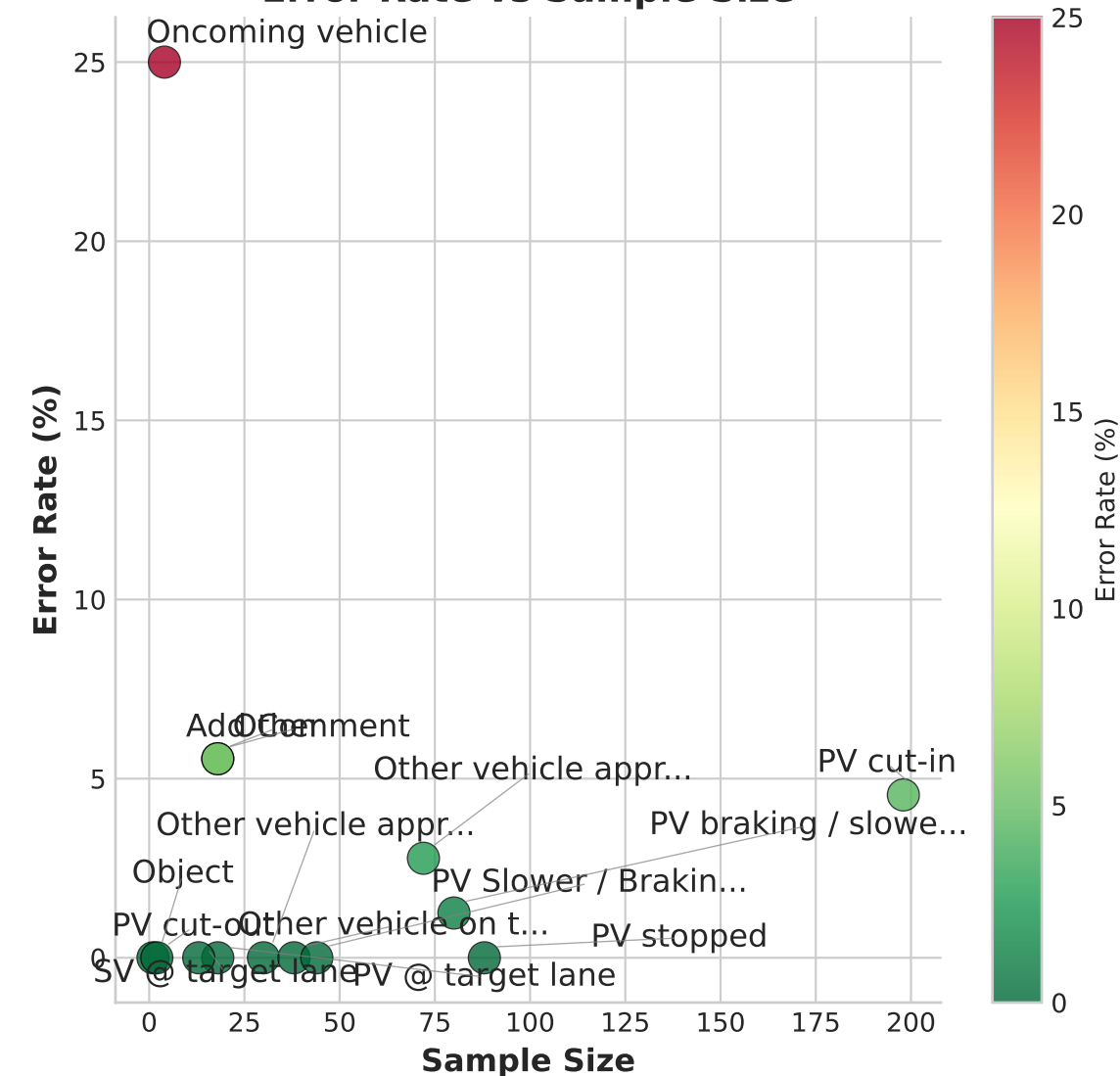
Error Rate vs Sample Size
