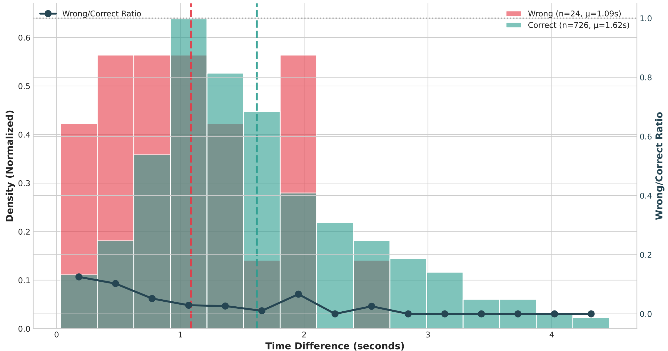
Time Difference Distribution (Normalized): Wrong vs Correct Predictions (with Error Ratio based on counts)
