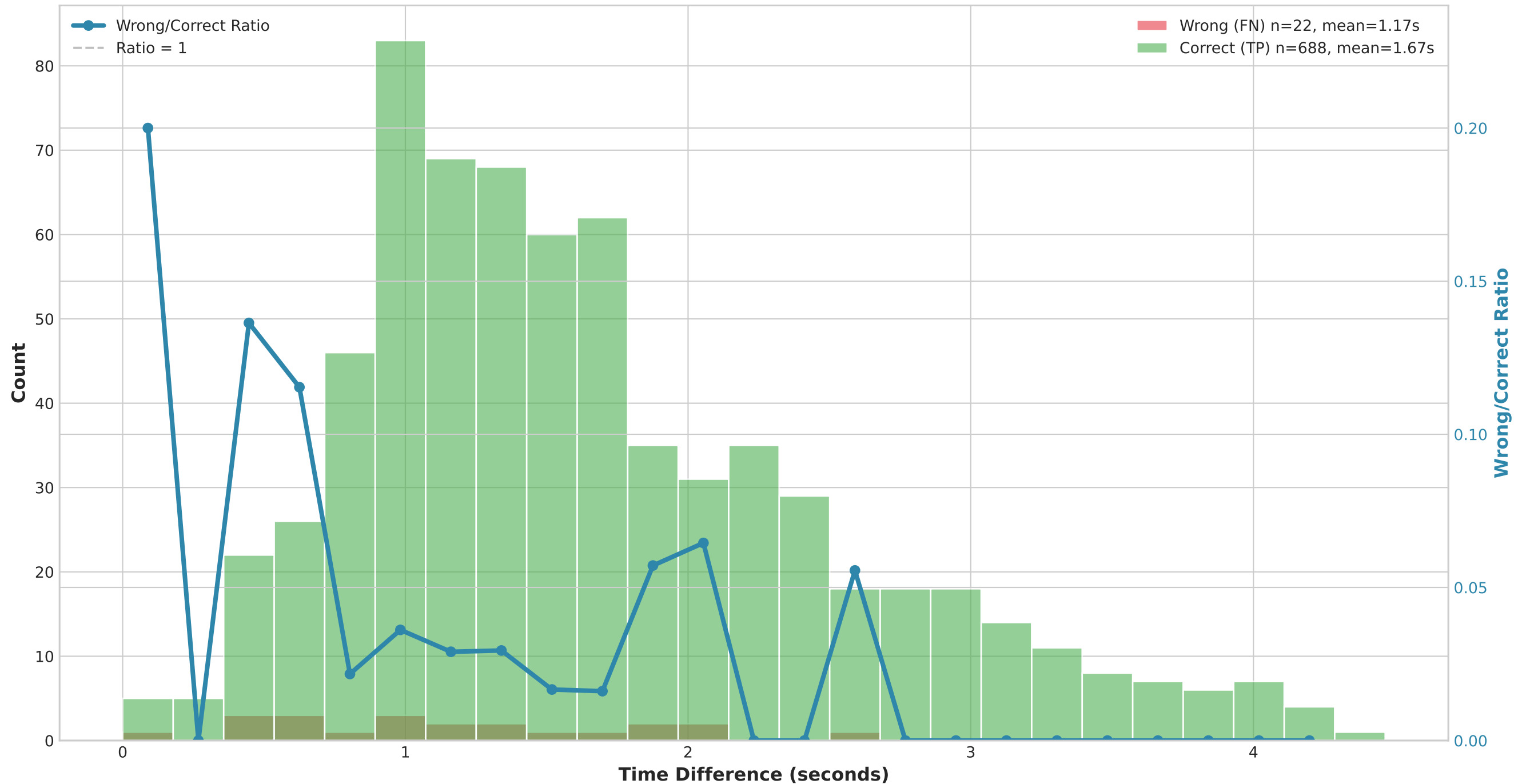
Time Difference: Wrong vs Correct Predictions (with Ratio Line) [VISIBLE ONLY SUBSET]
