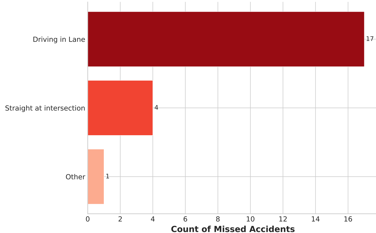
Missed Accidents by Scenario (Total FN: 22)
