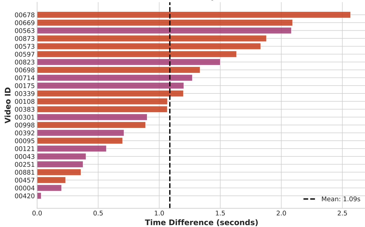
Time Difference by Video (Red=Val, Purple=Train)
