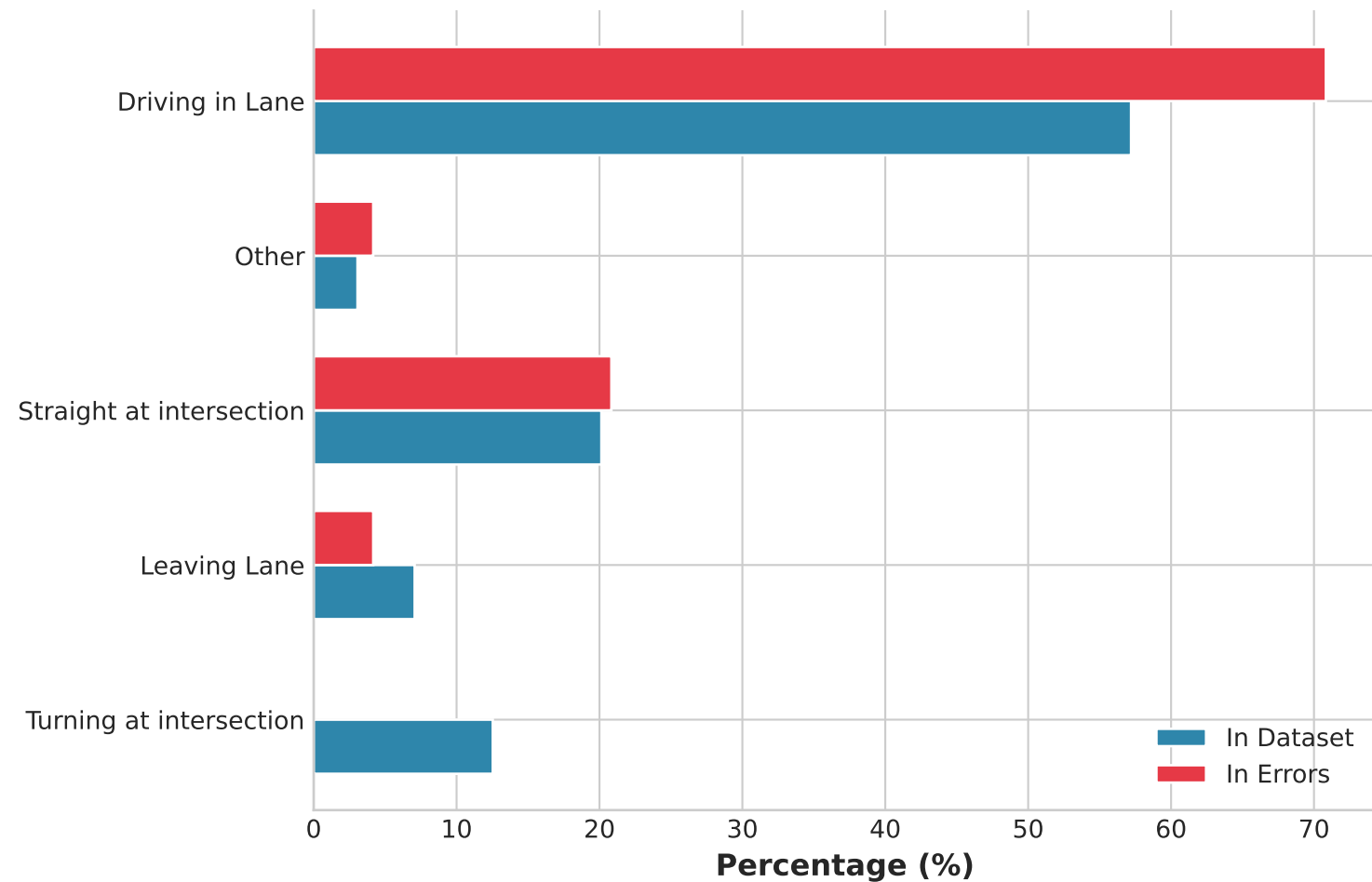
Dataset vs Error Distribution
