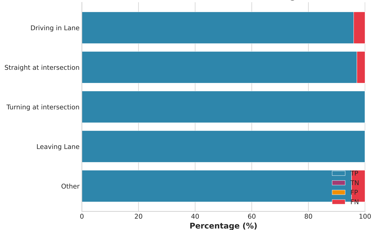
Prediction Outcome Percentages
