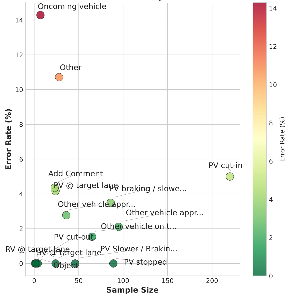
Error Rate vs Sample Size
