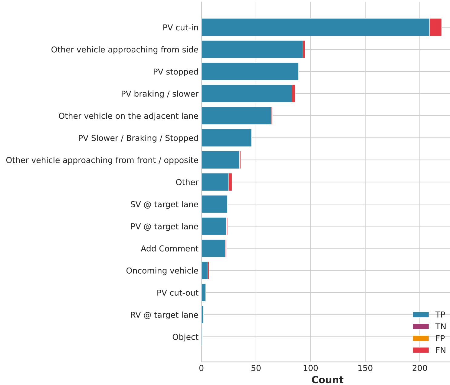
Prediction Outcome Counts
