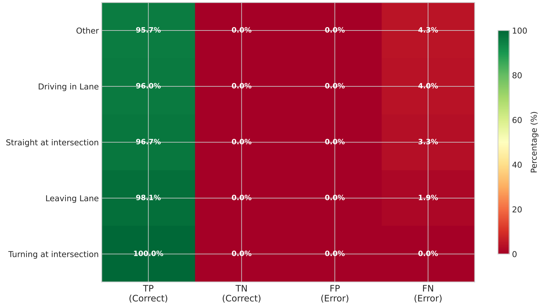
Prediction Outcome by Scenario (%) - Level 1 (Sorted by Error Rate)
