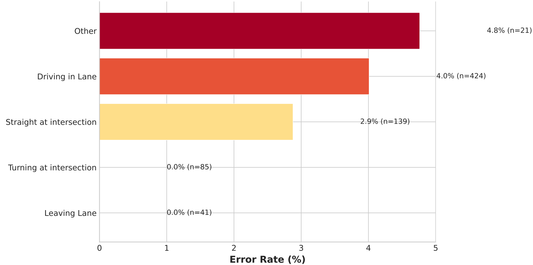
Error Rate per Scenario (Lower is Better)
