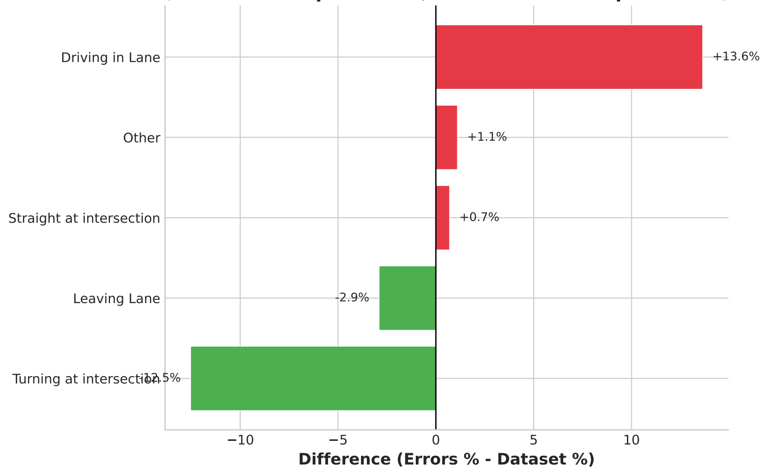
Over/Under-representation in Errors (Red = over-represented, Green = under-represented)
