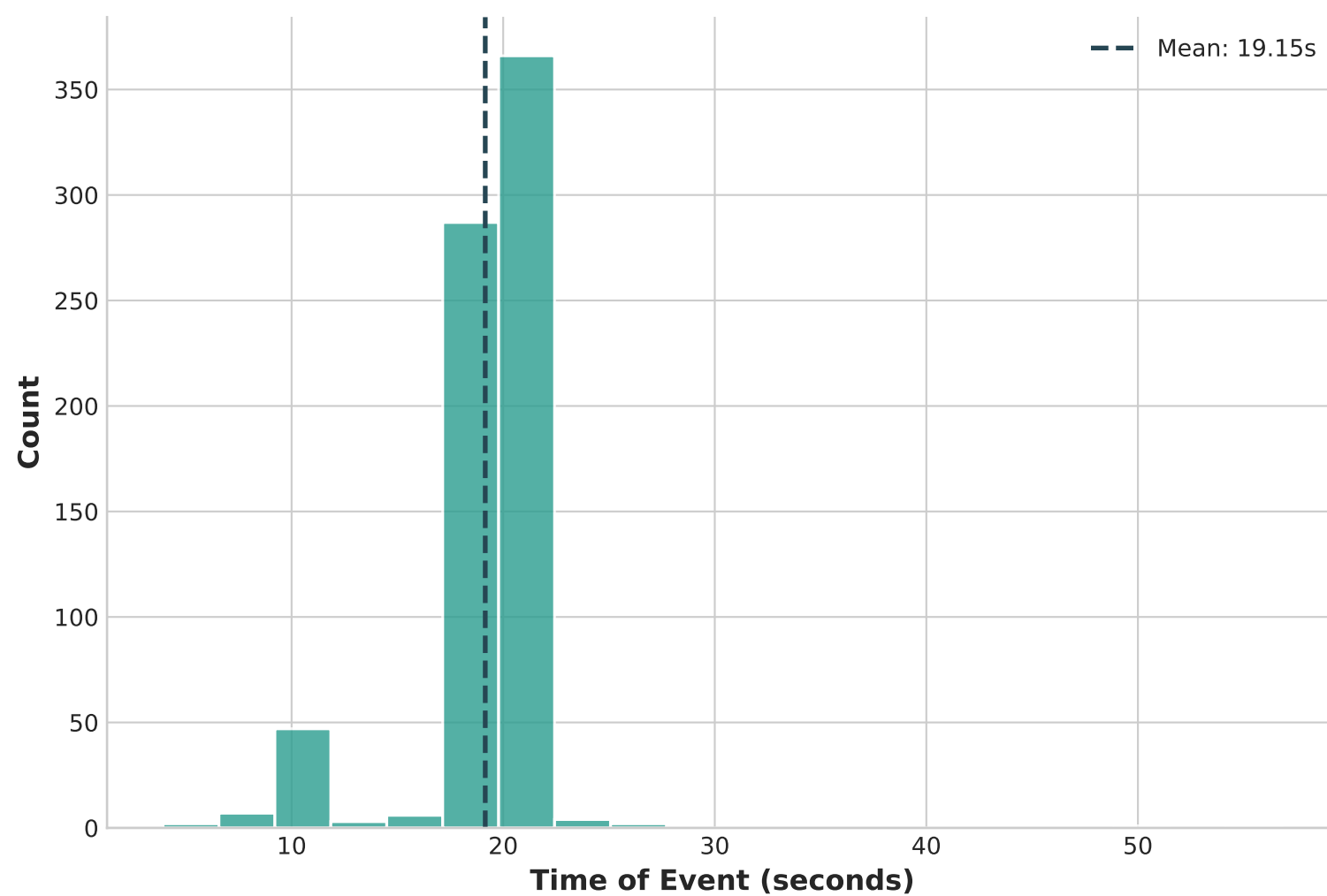
Distribution of Event Times
