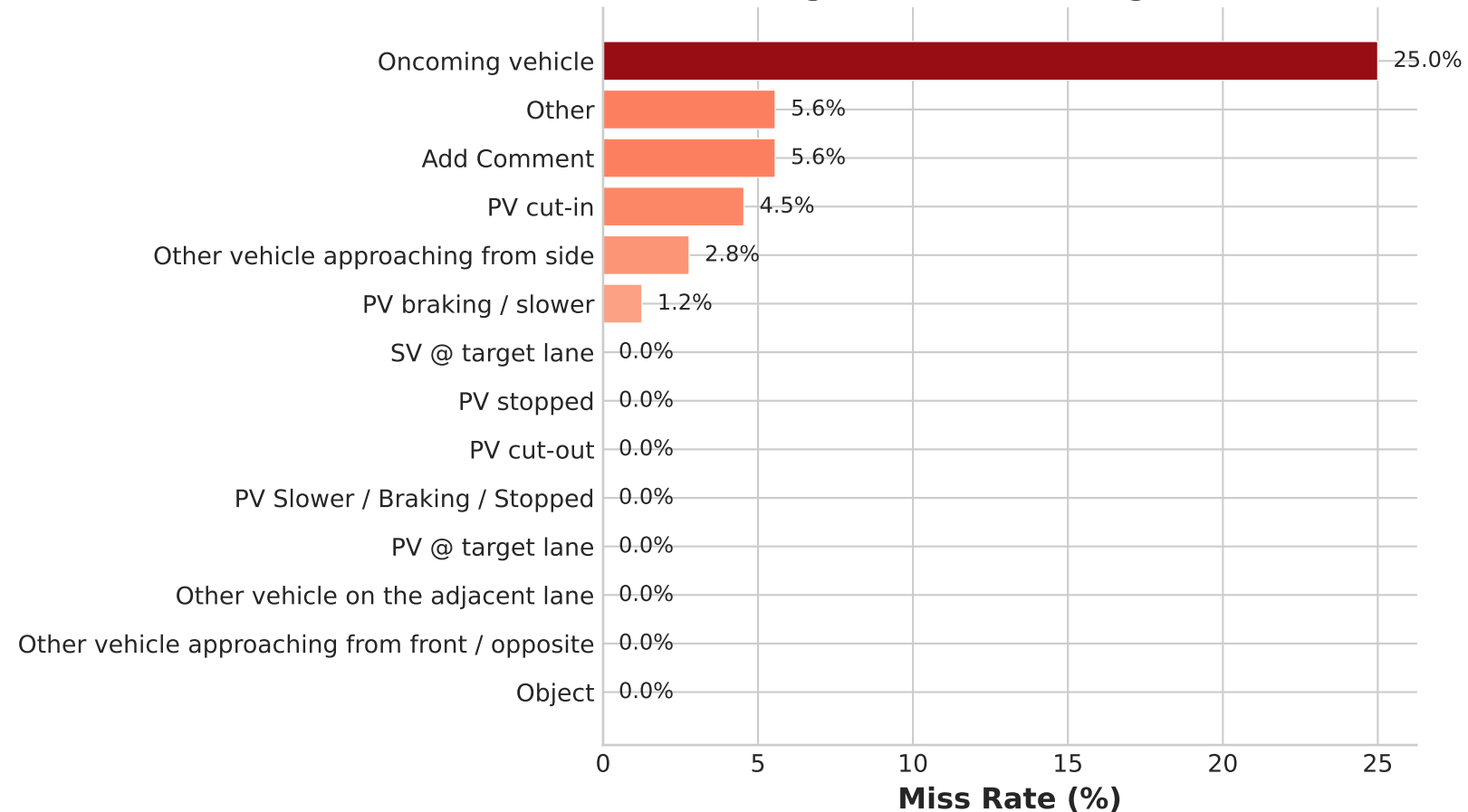
% of Positive Videos Missed (Higher = More Dangerous)
