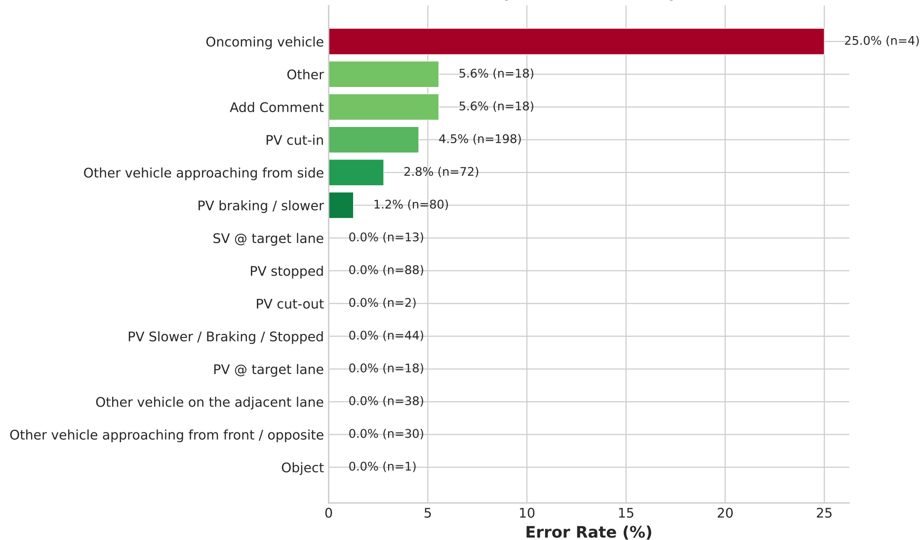
Error Rate per Scenario (Lower is Better)
