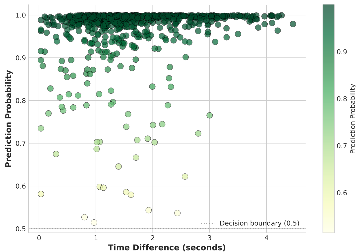
Time Difference vs Model Confidence (Correct Predictions)
