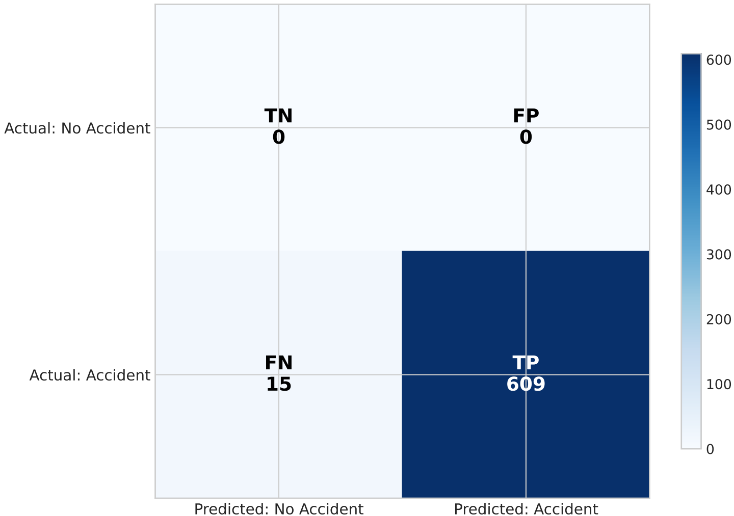
Confusion Matrix [VISIBLE ONLY - ALL]
