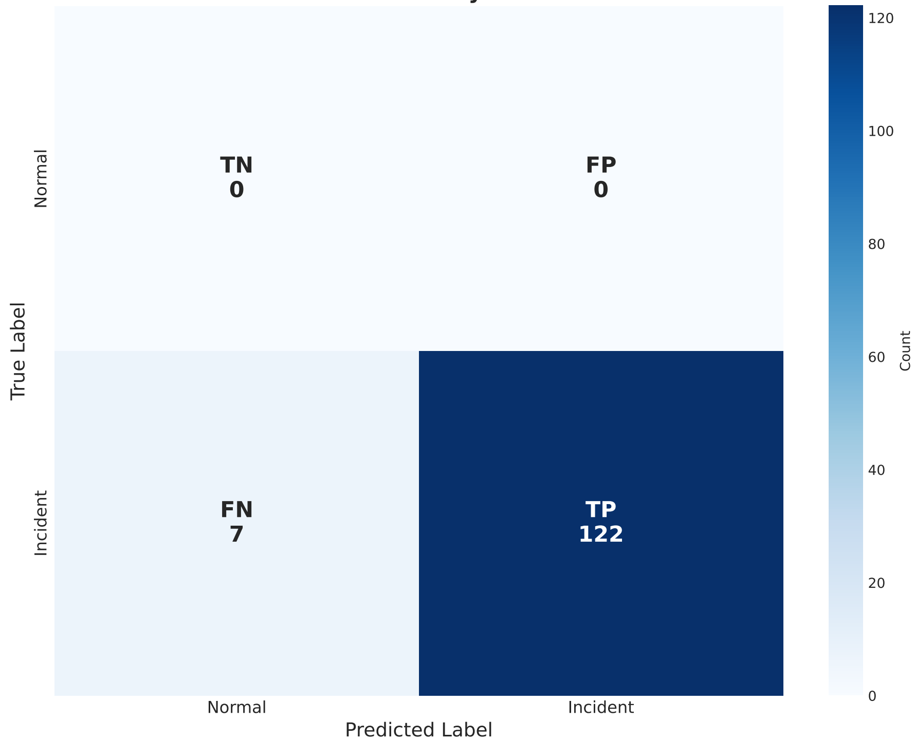
Confusion Matrix - Visible Only - Validation Dataset
