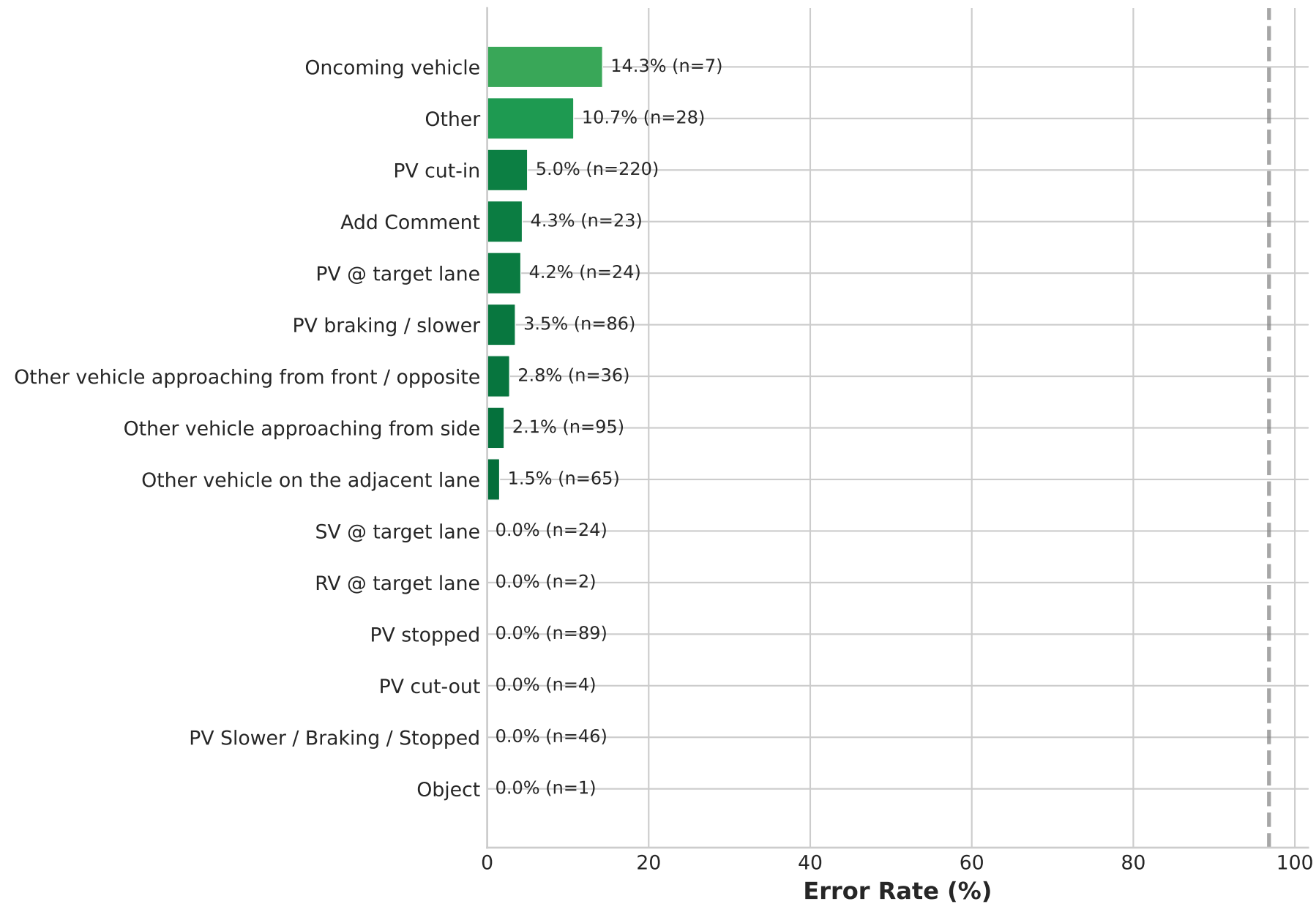
Error Rate per Scenario (Lower is Better)
