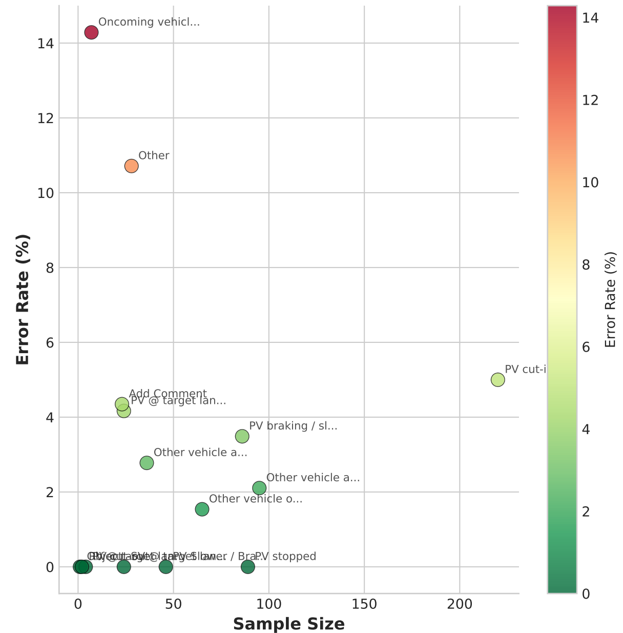
Error Rate vs Sample Size (Bubble = scenario)
