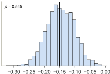
Quantum (109)
