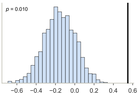
Quantum (109)
