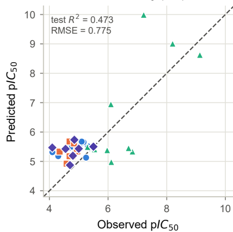
MACCS only (167)
