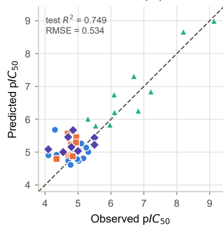
Pose 3D (112194)
