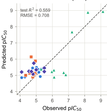
DFT quantum (109)
