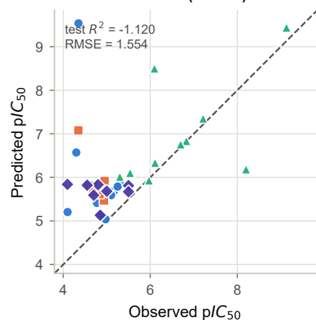
MACCS only (167)
