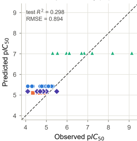
AlphaFold only (16)
