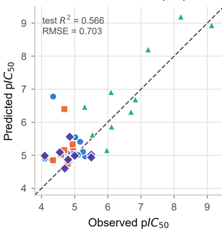
PaDEL 2D/3D (1444)
