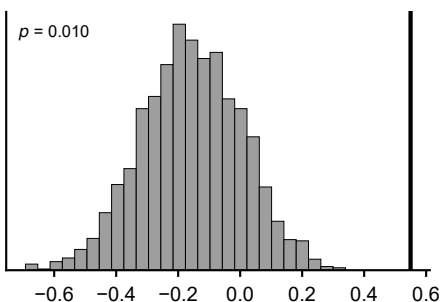
Quantum (109)
