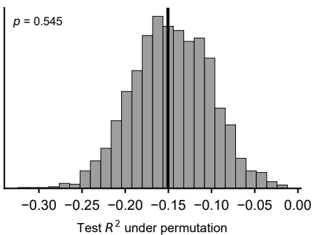
Quantum (109)
