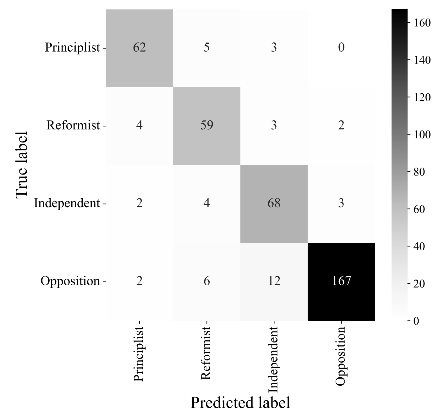
(f) Political websites n = 402 , Accuracy = 88.56%
