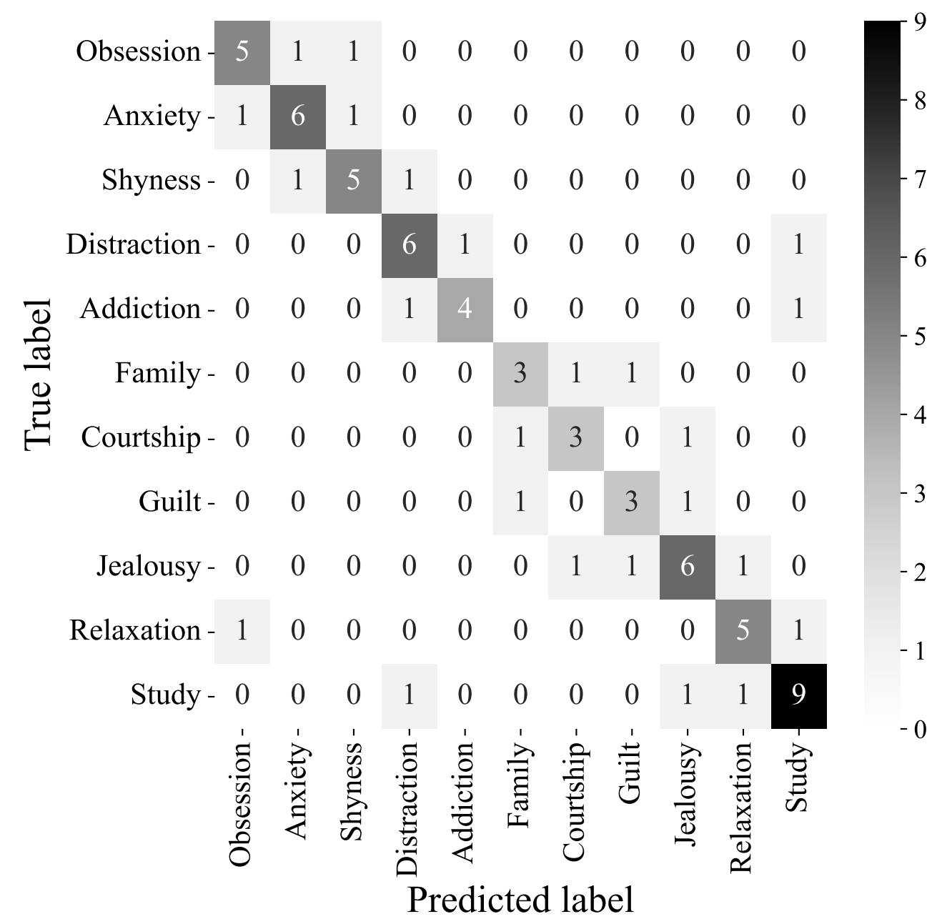
(d) Psychological advise n = 79 , Accuracy = 69.62%
