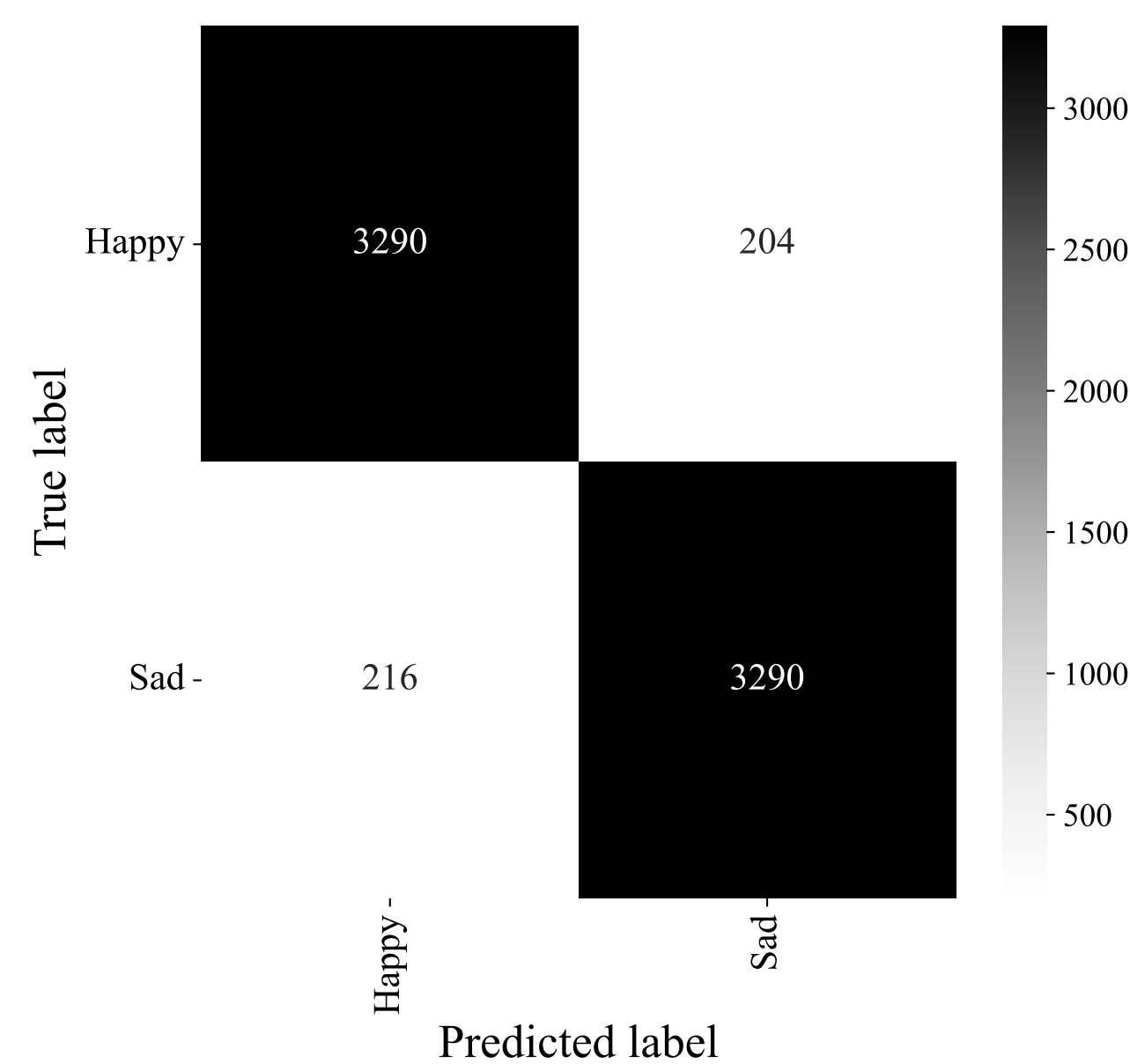
(e) Snappfood n = 7000 , Accuracy = 94.00%
