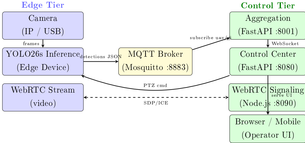
Figure 3.1: System architecture overview. Edge nodes run YOLO26s inference locally and publish detection results over MQTT to the control center. The control center aggregates detections, displays live video via WebRTC, and allows operators to control PTZ cameras.
