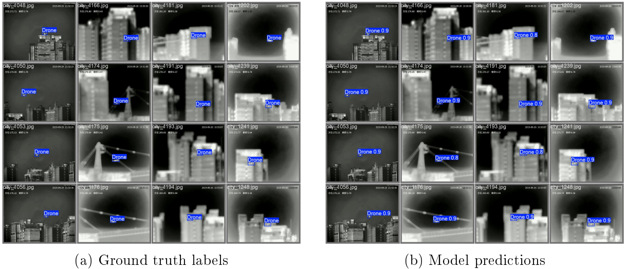
Figure 4.8: ThermalDrone validation batch 0: ground truth (left) vs model predictions (right). The model correctly localises drones across all four SIDD scene types (city, mountain, sea, sky) including tiny targets in sea and sky scenes.
