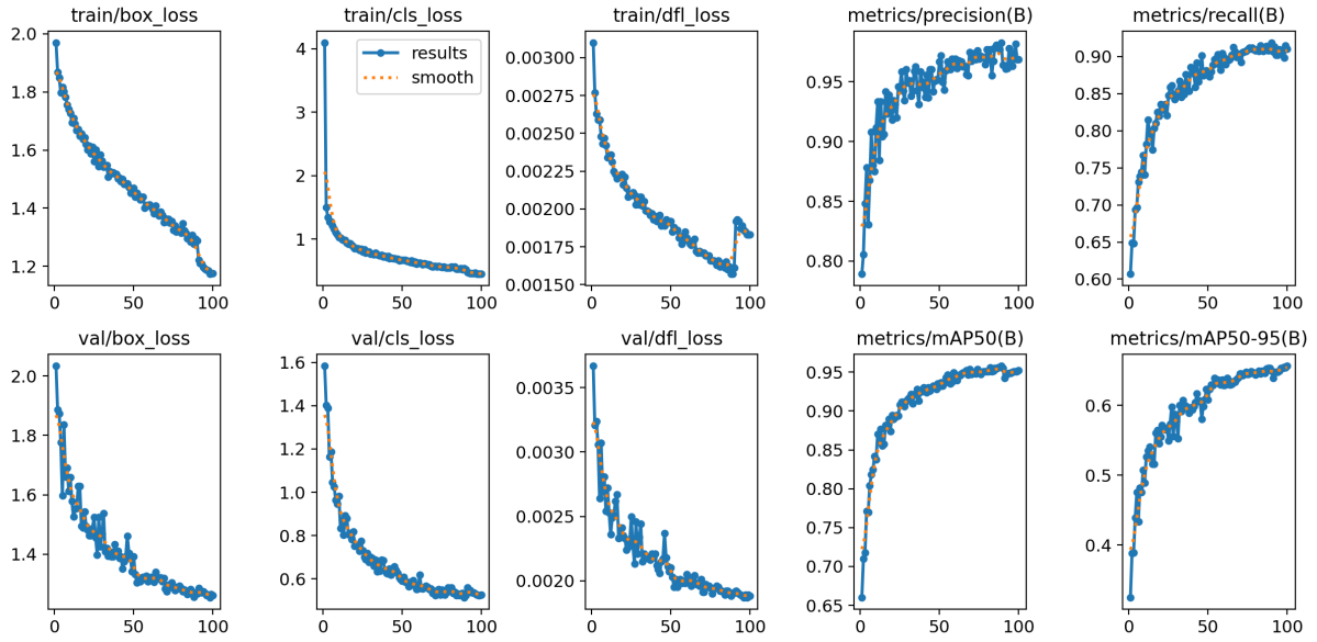
Figure 4.5: ThermalDrone training curves (100 epochs, RTX 2070). mAP@0.5 rises from 0.660 at epoch 1 to 0.837 at epoch 10, reaches 0.946 at epoch 55, and peaks at 0.958 at epoch 89. Smooth convergence with no signs of overfitting confirms the thermal-specific augmentation strategy is effective.
