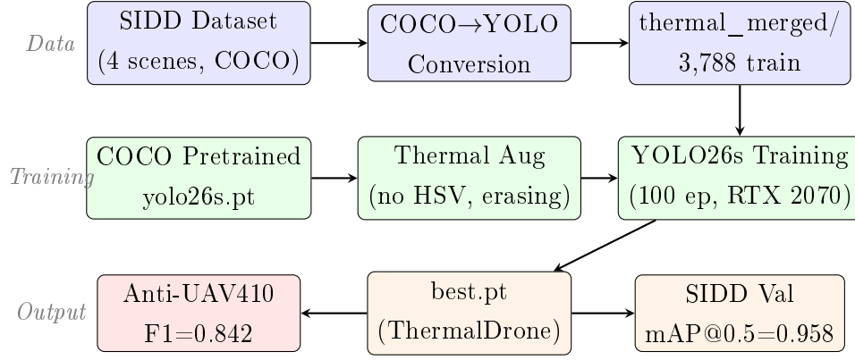
Figure 4.4: ThermalDrone pipeline. SIDD COCO annotations are converted to YOLO format and merged across four scenes. Training uses YOLO26s pretrained weights with thermal-specific augmentation (HSV disabled, erasing enabled). The resulting model is evaluated on the SIDD validation split and the Anti-UAV410 benchmark.
