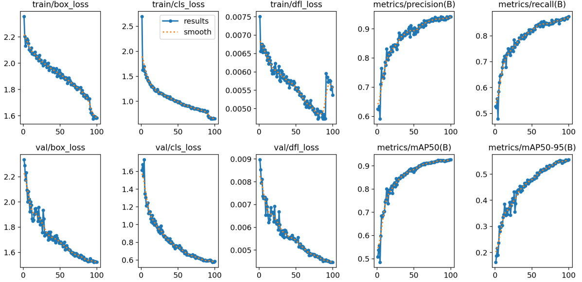
Figure 4.1: BirdDrone-2C base training curves (100 epochs, local training). Smooth convergence with \text{mAP}@0.5 reaching 0.926 at epoch 99. The base model provides the starting weights for fine-tuning.
