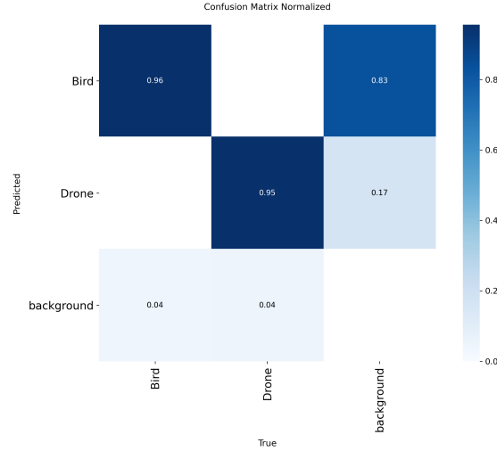
Figure 4.3: BirdDrone-2C fine-tuned model normalised confusion matrix. The Bird→Drone false alarm rate remains at 0.3%, identical to the base model, confirming fine-tuning did not introduce new false positive behaviour.
