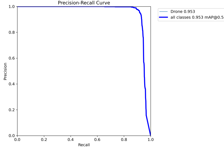
Figure 4.8: ThermalDrone Precision-Recall curve on SIDD validation split. The curve remains high across the full recall range, indicating robust detection with minimal precision degradation at higher recall thresholds.
