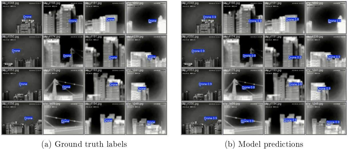
Figure 4.9: ThermalDrone validation batch 0: ground truth (left) vs model predictions (right). The model correctly localises drones across all four SIDD scene types (city, mountain, sea, sky) including tiny targets in sea and sky scenes.
