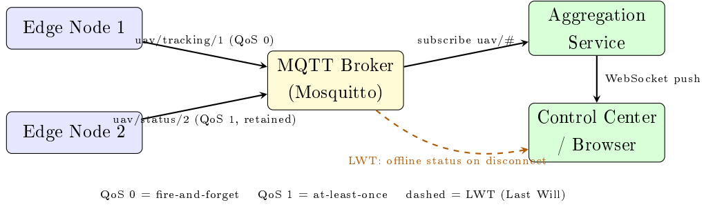
Figure 3.3: MQTT publish-subscribe flow. Edge nodes publish detection results ( uav/tracking/{id} ) at up to 25 fps (QoS 0) and status messages ( uav/status/{id} ) as retained messages (QoS 1). The aggregation service subscribes to all uav/# topics and pushes updates to the control center via WebSocket. The Last Will and Testament (LWT) mechanism automatically publishes an offline status if an edge device disconnects unexpectedly.
