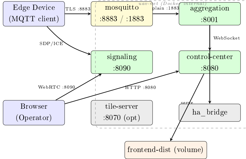
Figure 3.2: Docker services architecture. All server-side services run inside the uav-net Docker network. Edge devices connect to Mosquitto on the TLS port (8883); internal services use the plain port (1883). The frontend-dist volume is written by the builder and served by the control center.
