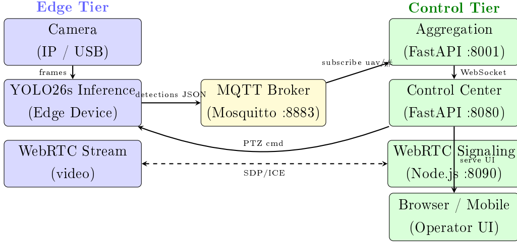
Figure 3.1: System architecture overview. Edge nodes run YOLO26s inference locally and publish detection results over MQTT to the control center. The control center serves the web UI directly to the browser (HTTP), independent of the WebRTC signaling path. WebRTC video flows from the edge device through the signaling server for SDP/ICE negotiation, then streams peer-to-peer to the browser. PTZ commands flow from the control center back to the edge device via MQTT.
