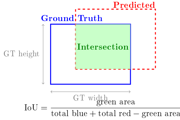
Figure 4.4: Illustration of Intersection over Union (IoU). The green region is the intersection of the predicted (red dashed) and ground-truth (blue solid) bounding boxes. IoU is the ratio of the intersection area to the union area. A detection is a true positive when \text{IoU} \geq \tau (typically \tau = 0.5 ).
