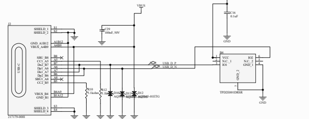
USB-C Connector - 2
