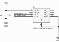
Cryptographic Co-Processor
