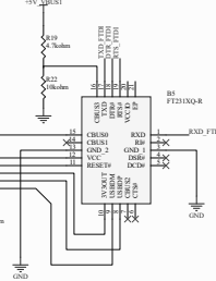
USB To UART
