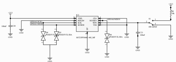
Serial Quad I/O Flash Memory with Write Protection Switch
