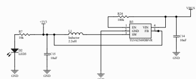
Step-down Buck Converter
