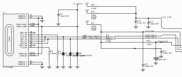
USB-C Connector - 1
