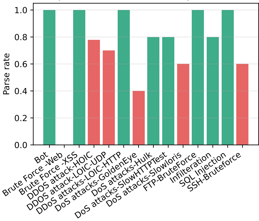
JSON Parse Success Rate per Class
