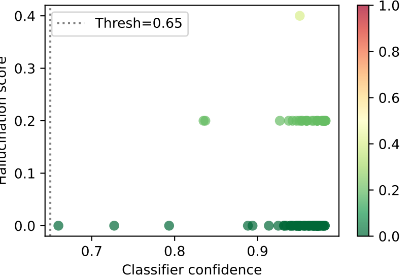
Confidence vs Hallucination
